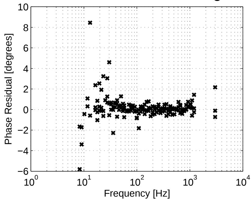
Statistical Variance in Sensing Phase
