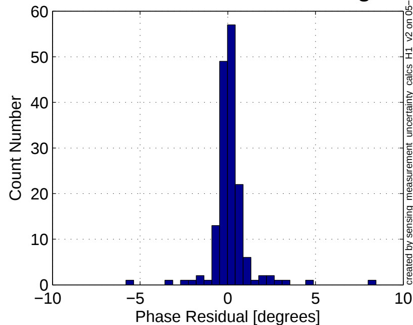
Phase Res -- Std: 1.16 degrees
