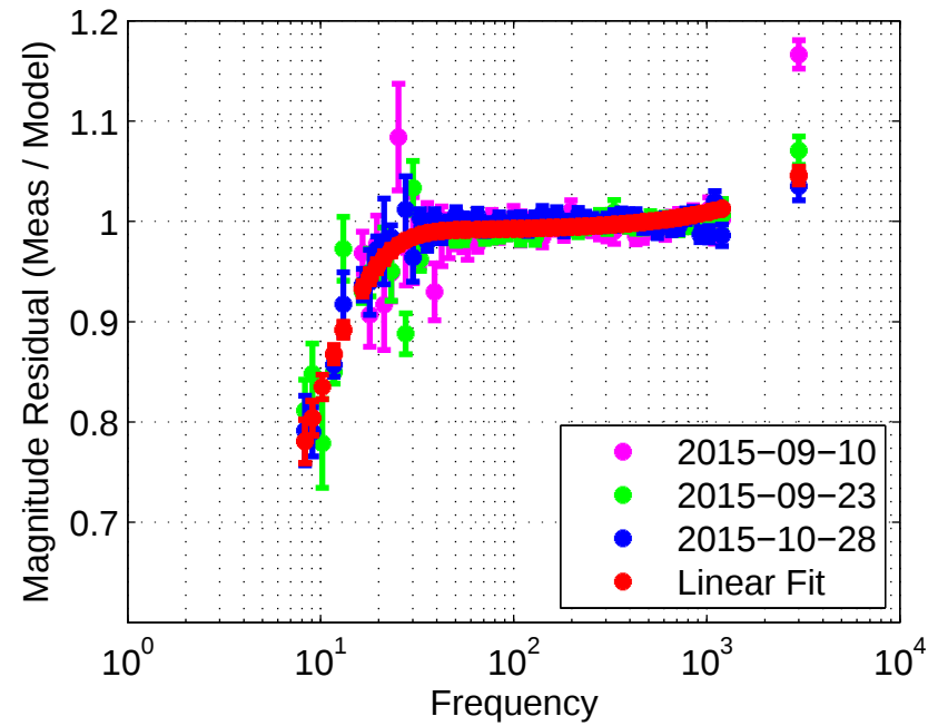
Magnitude Residuals with errorbars
