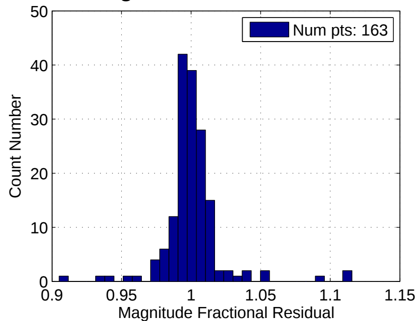
Mag Res -- Std: 0.0119
