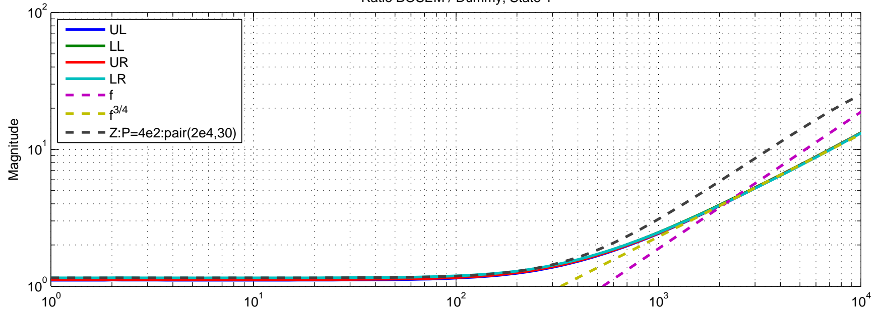
Ratio BOSEM / Dummy, State 1
