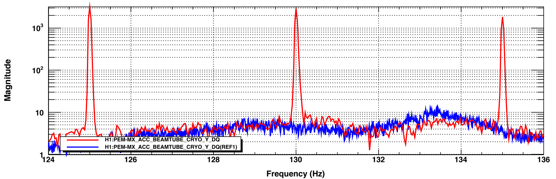
Mid-X beam tube accelerometer, BLUE: nominal, RED: speaker injection
