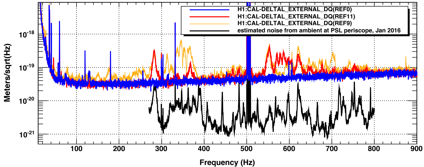
DARM, BLUE: no inject, RED: Jan 2016, injection, ORANGE: Sept. 2015 same amplitude injection
