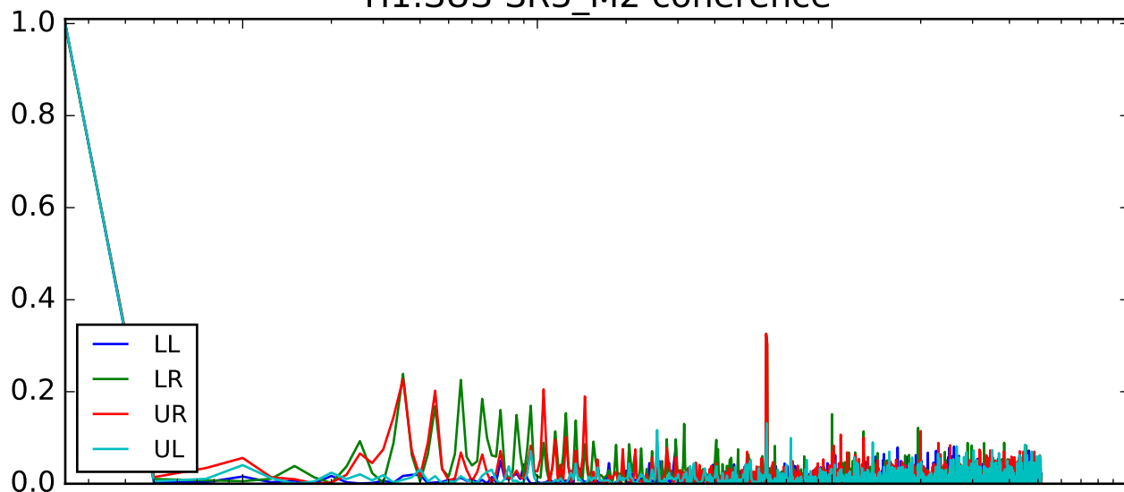
H1:SUS-SR3_M2 coherence
