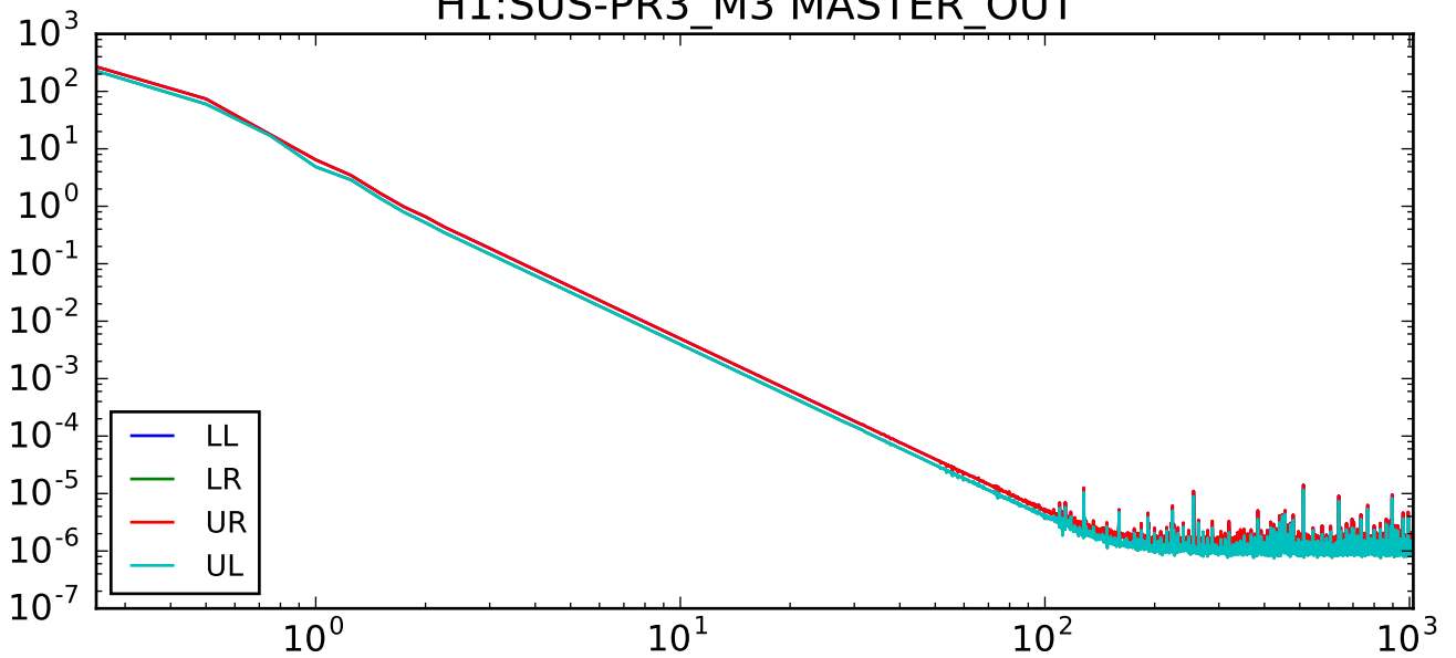
H1:SUS-PR3_M3 MASTER_OUT
