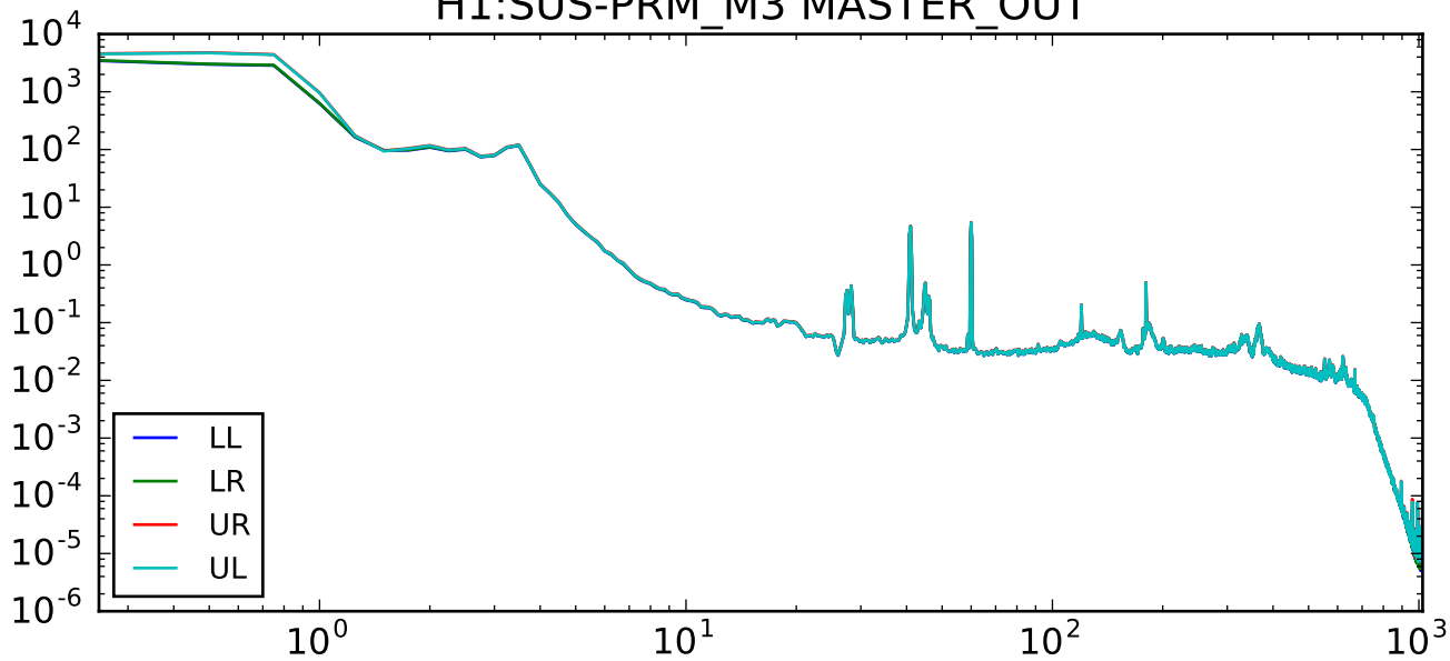
H1:SUS-PRM_M3 MASTER_OUT
