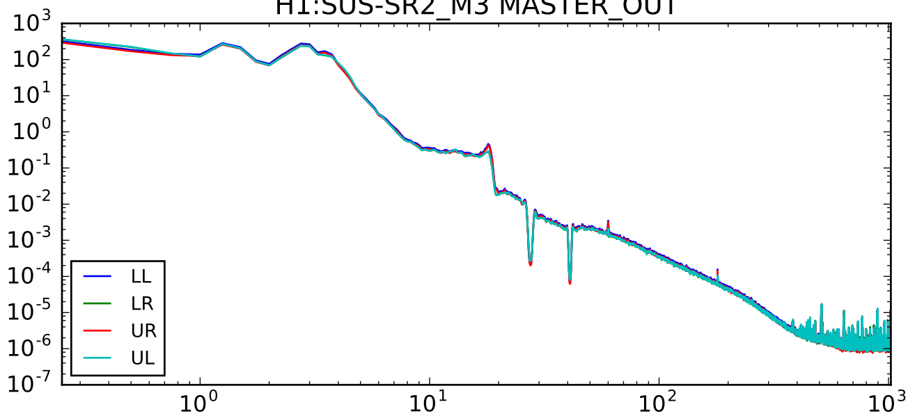
H1:SUS-SR2_M3 MASTER_OUT
