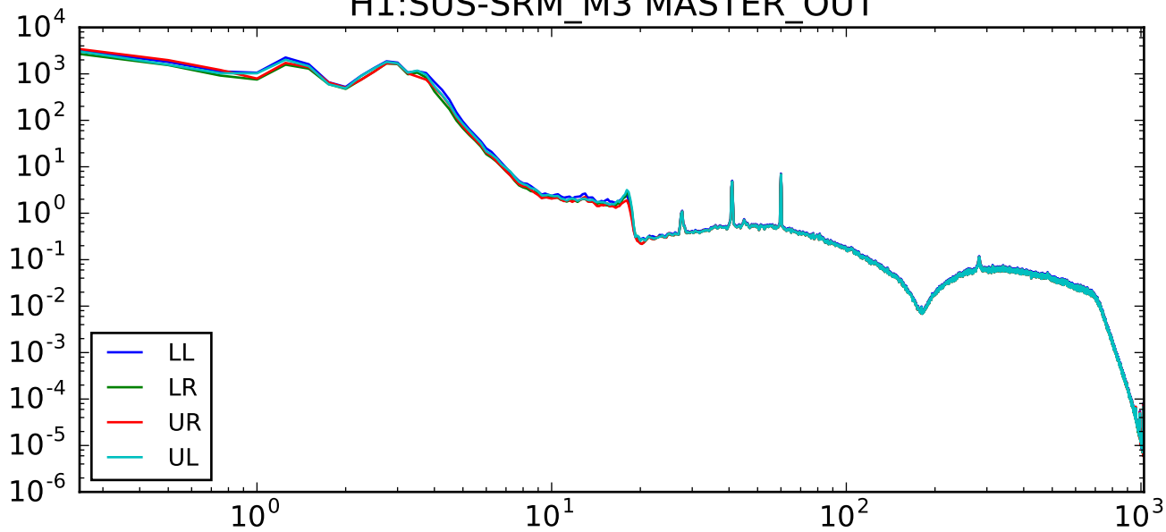
H1:SUS-SRM_M3 MASTER_OUT
