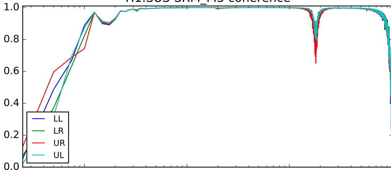
H1:SUS-SRM_M3 coherence
