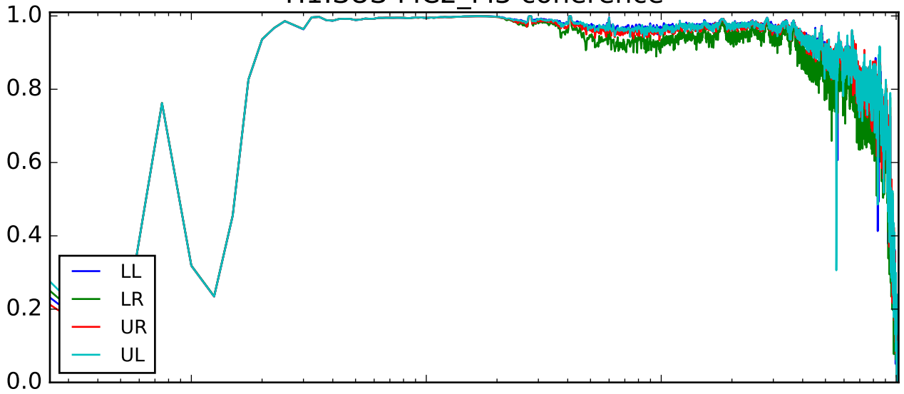
H1:SUS-MC2_M3 MASTER_OUT
