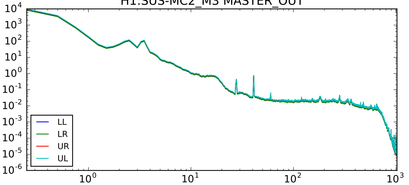
H1:SUS-MC2_M3 MASTER_OUT
