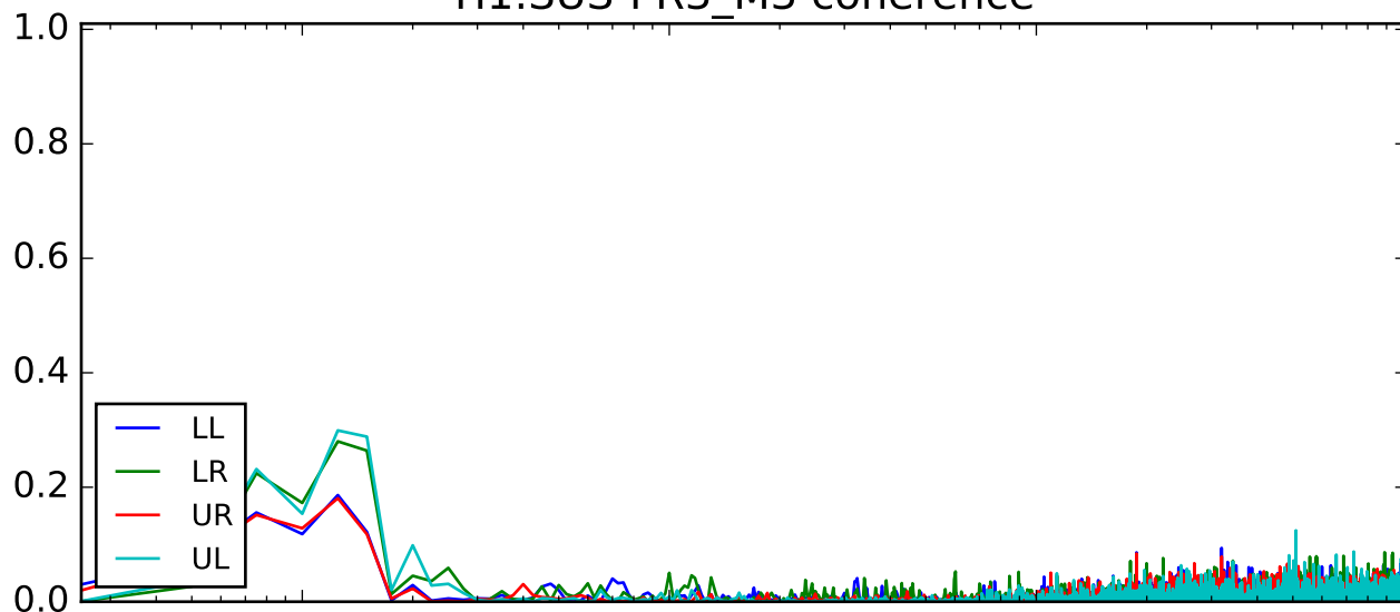
H1:SUS-PR3_M3 coherence
