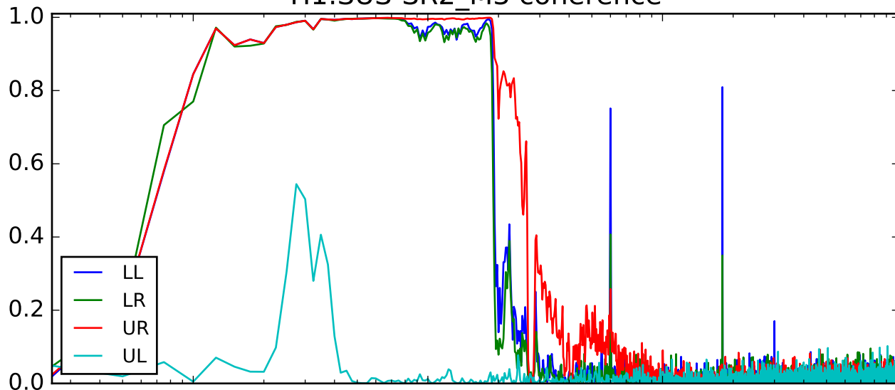
H1:SUS-SR2_M3 coherence
