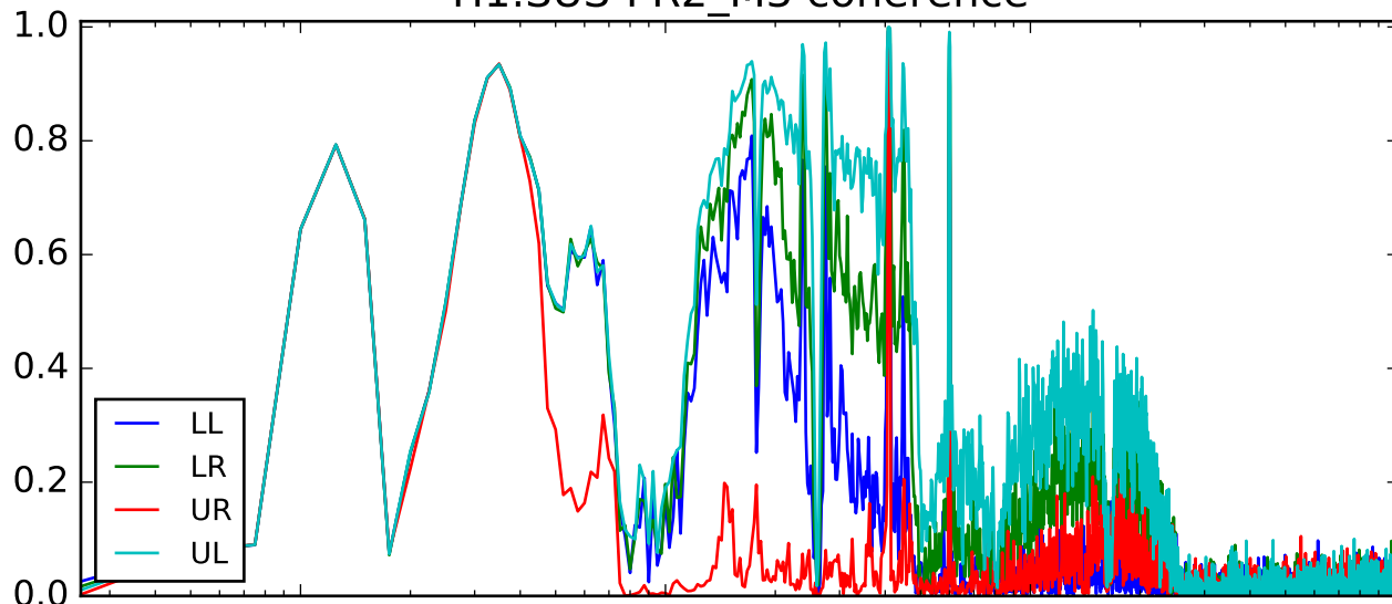
H1:SUS-PR2_M3 coherence
