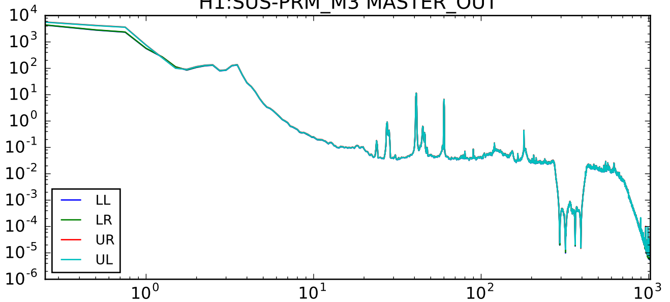
H1:SUS-PRM_M3 MASTER_OUT
