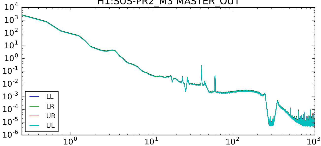
H1:SUS-PR2_M3 MASTER_OUT
