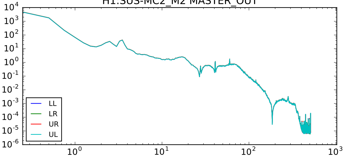
H1:SUS-MC2_M2 MASTER_OUT
