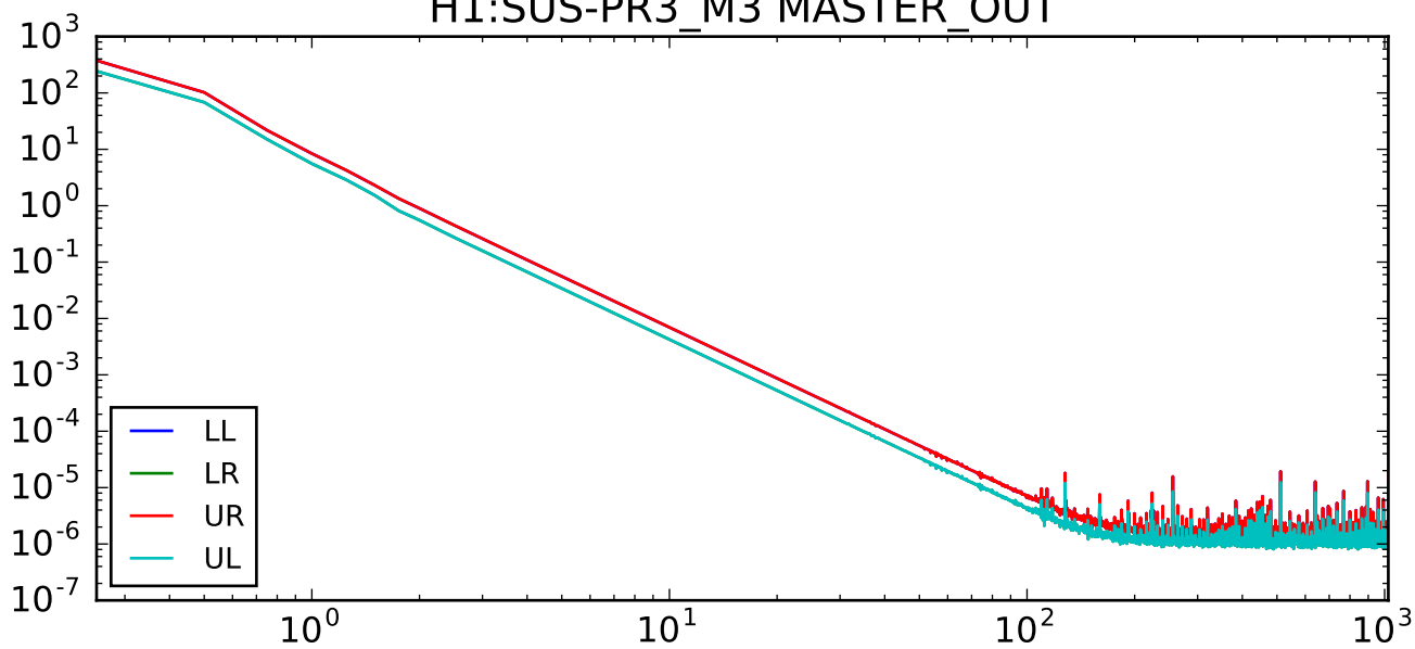
H1:SUS-PR3_M3 MASTER_OUT
