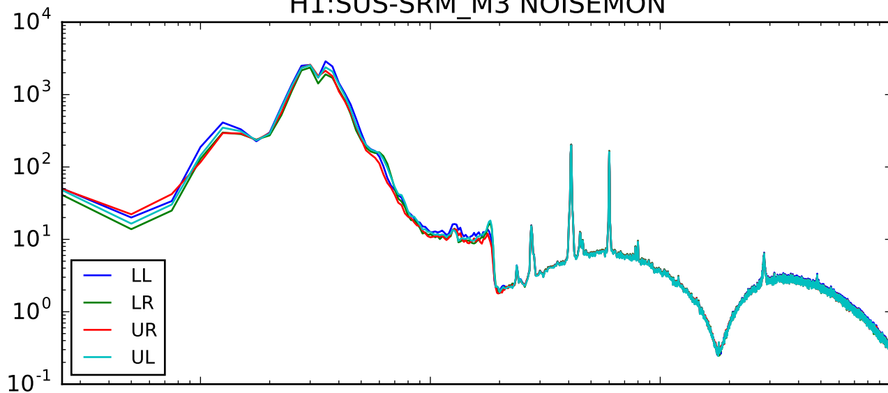
H1:SUS-SRM_M3 coherence
