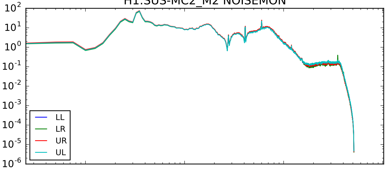
H1:SUS-MC2_M2 coherence
