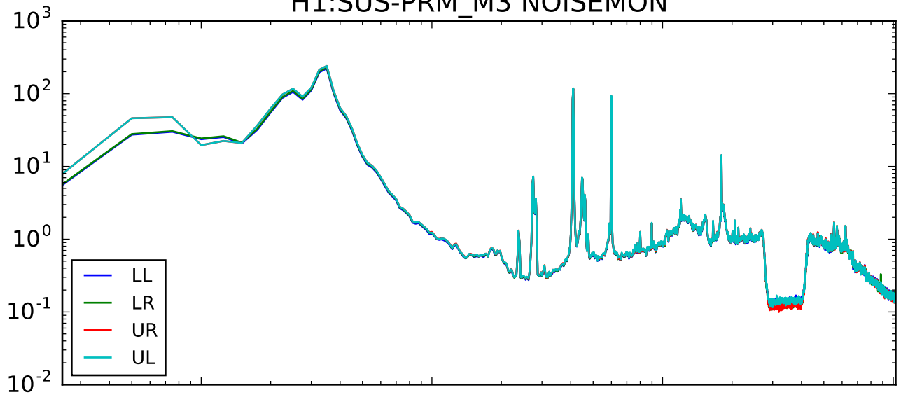
H1:SUS-PRM_M3 coherence
