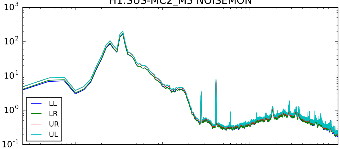
H1:SUS-MC2_M3 coherence
