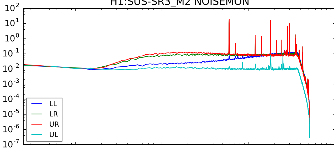
H1:SUS-SR3_M2 coherence
