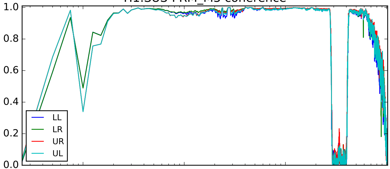
H1:SUS-PRM_M3 MASTER_OUT
