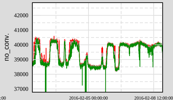
Ch 7: H1:SUS-SR3_M3_OPLEV_SUM_OUT16
