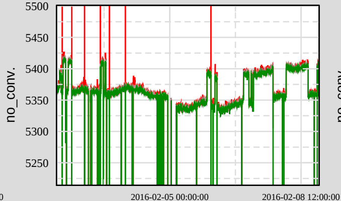
Ch 4: H1:SUS-ITMY_L3_OPLEV_SUM_OUT16
