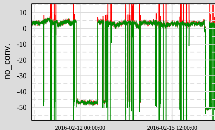
Ch 1: H1:SUS-ETMX_L3_OPLEV_PIT_OUT16
