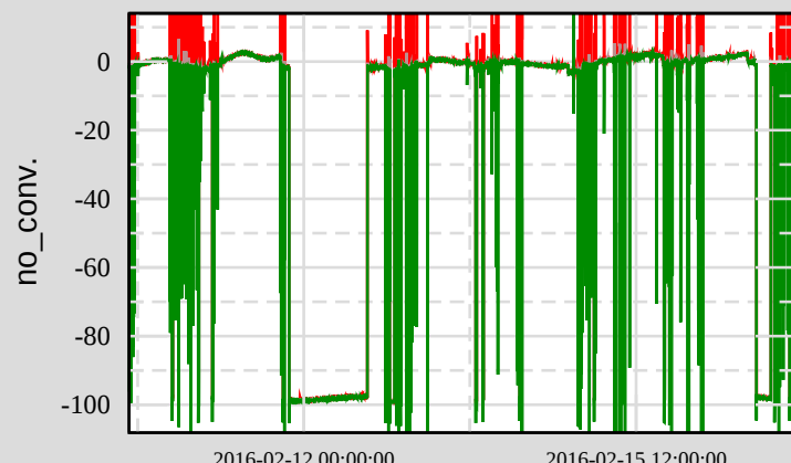
Ch 1: H1:SUS-ETMX_L3_OPLEV_PIT_OUT16
