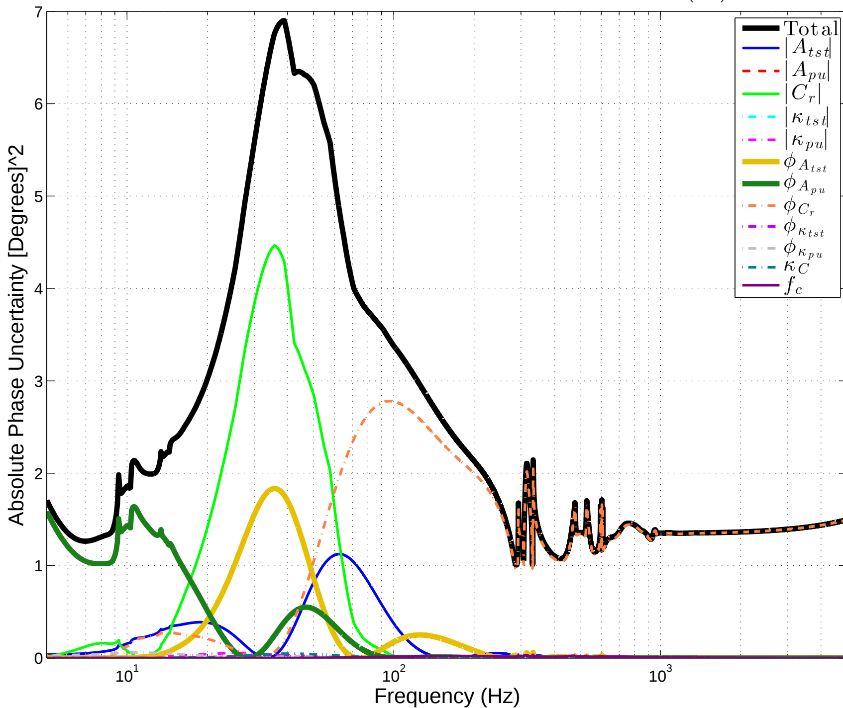
LHO C01 Squared Phase Uncertainty Components \left(\frac{\partial \phi_h}{\partial x_i}\right)^2 \sigma_{x_i}^2
