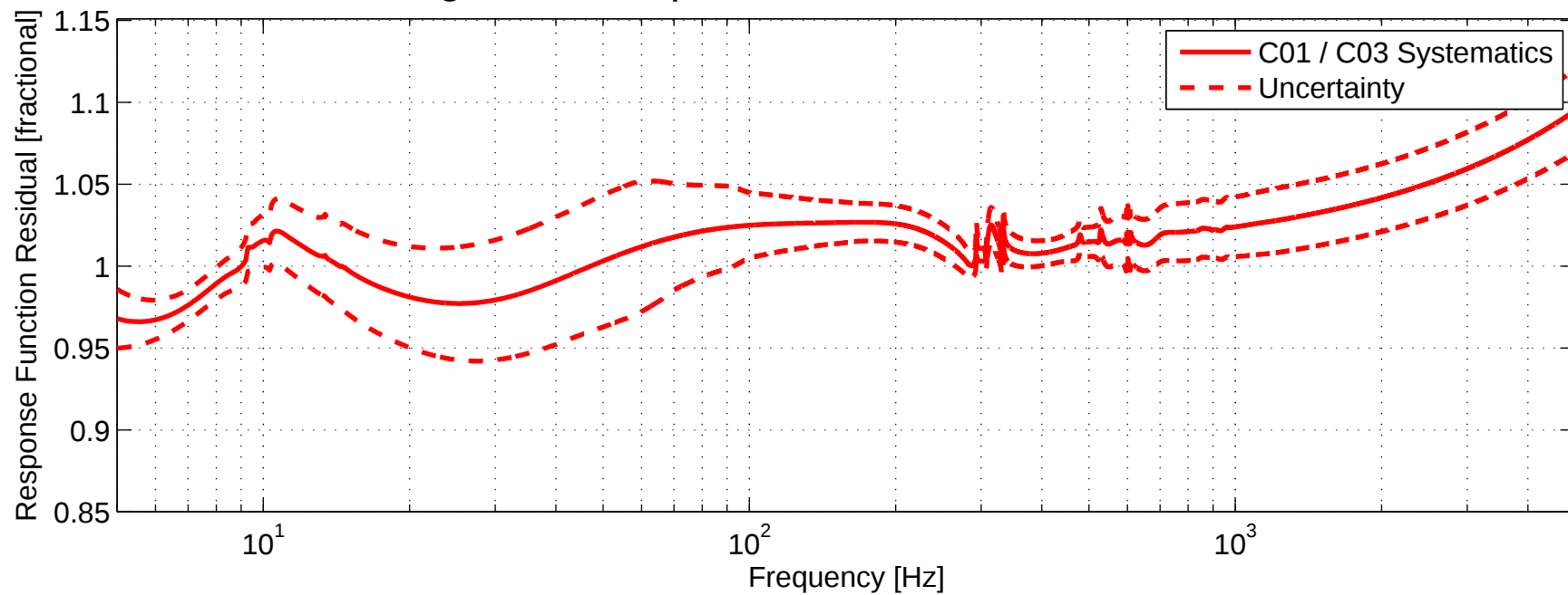
LHO C01 Magnitude Response Function – GPS Time = 1126259461
