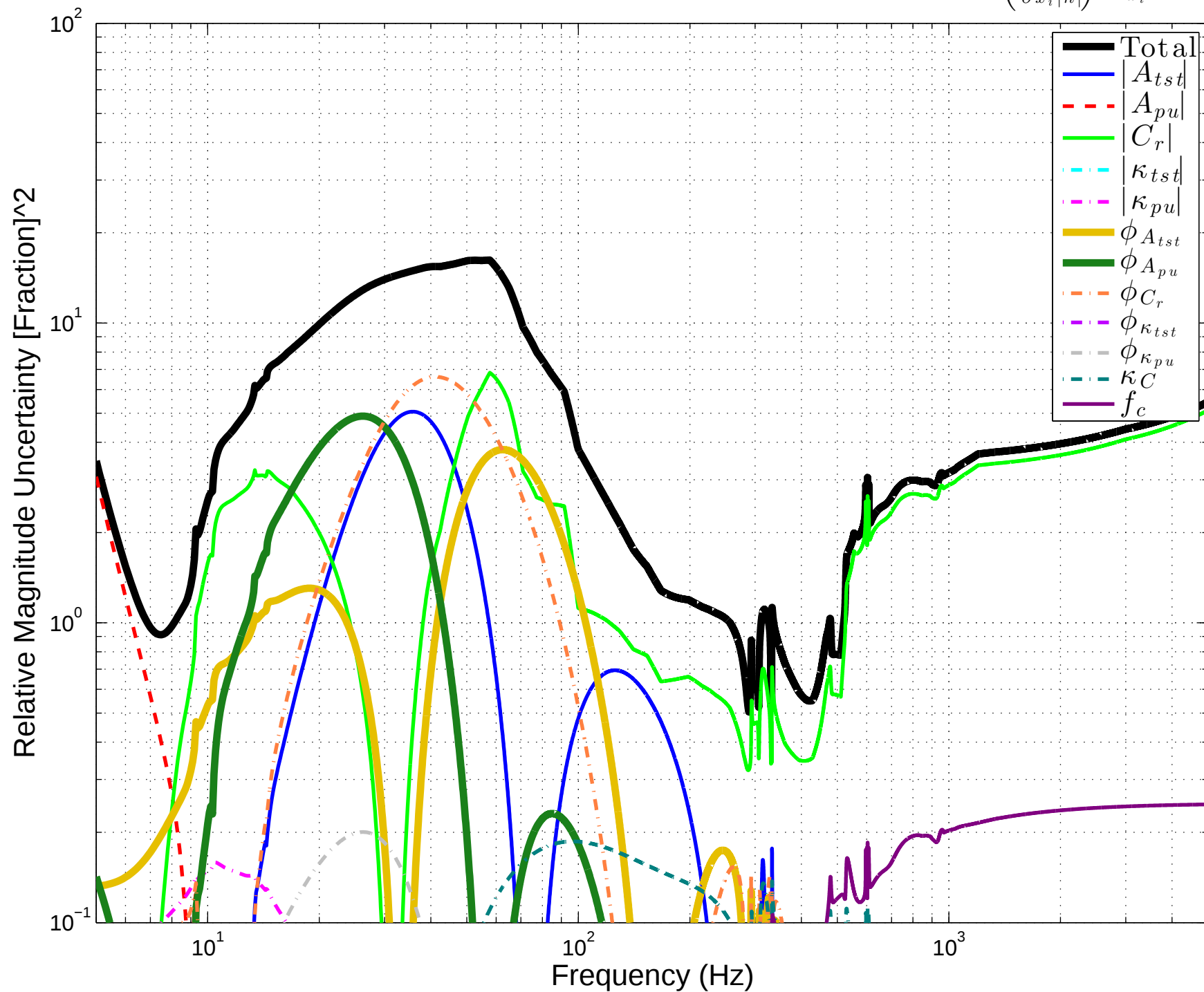
LHO C01 Squared Magnitude Uncertainty Components \left(\frac{\partial |h|}{\partial x_i} \frac{1}{|h|}\right)^2 \sigma_{x_i}^2
