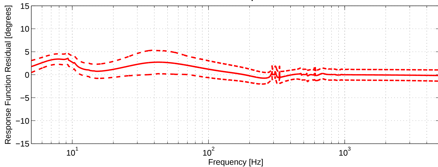
LHO C01 Phase Response Function
