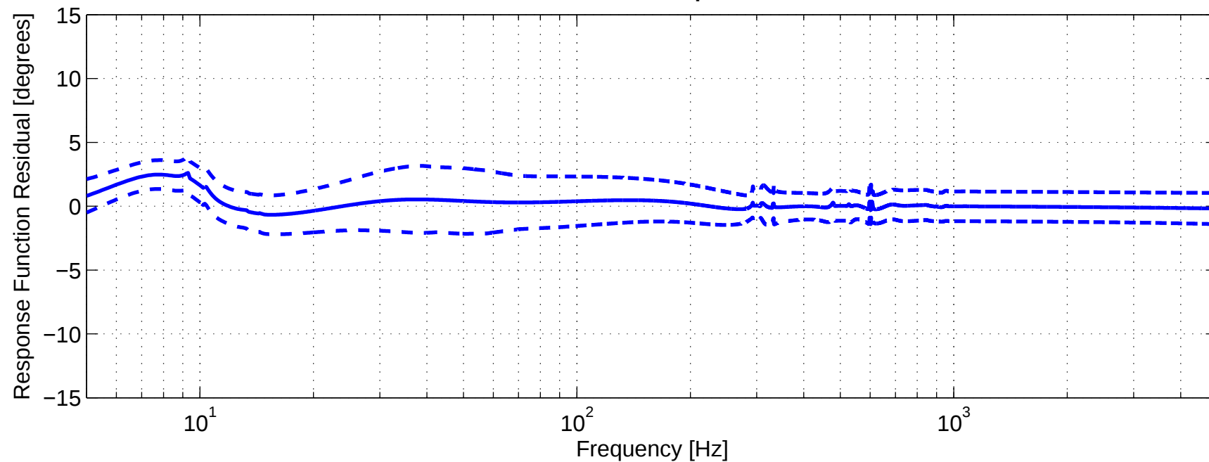
LHO C02 Phase Response Function
