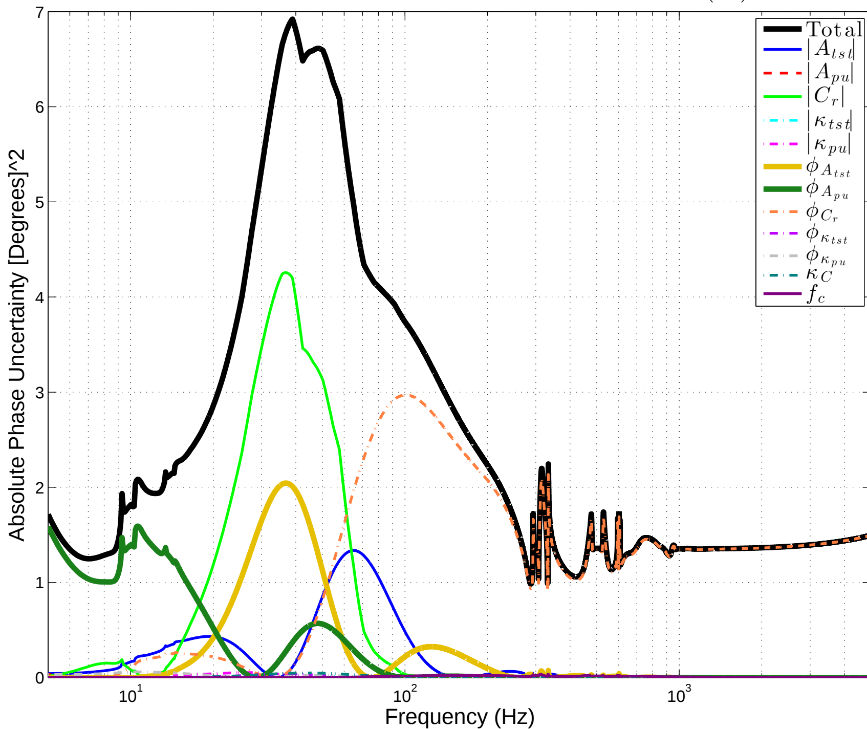
LHO C02 Squared Phase Uncertainty Components \left(\frac{\partial \phi_h}{\partial x_i}\right)^2 \sigma_{x_i}^2
