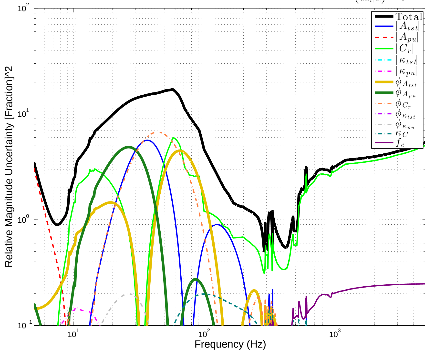
LHO C02 Squared Magnitude Uncertainty Components \left(\frac{\partial |h|}{\partial x_i} \frac{1}{|h|}\right)^2 \sigma_{x_i}^2
