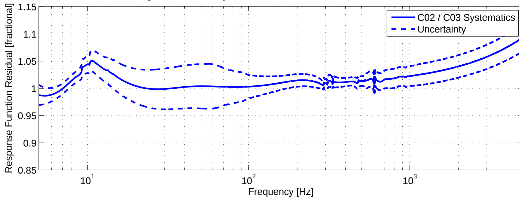
LHO C02 Magnitude Response Function – GPS Time = 1126259461
