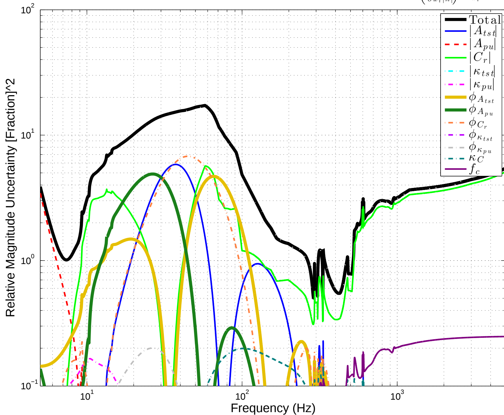
LHO C03 Squared Magnitude Uncertainty Components \left(\frac{\partial|h|}{\partial x_i|h|}\right)^2 \sigma_{x_i}^2
