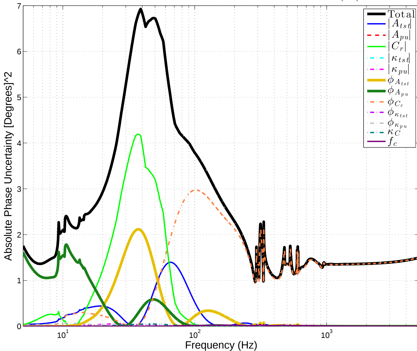
LHO C03 Squared Phase Uncertainty Components \left(\frac{\partial \phi_h}{\partial x_i}\right)^2 \sigma_{x_i}^2
