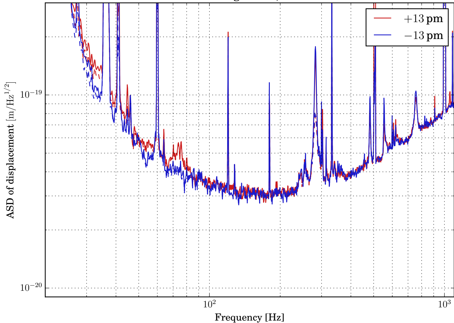
DARM offset sign tests, 2016-02-21
