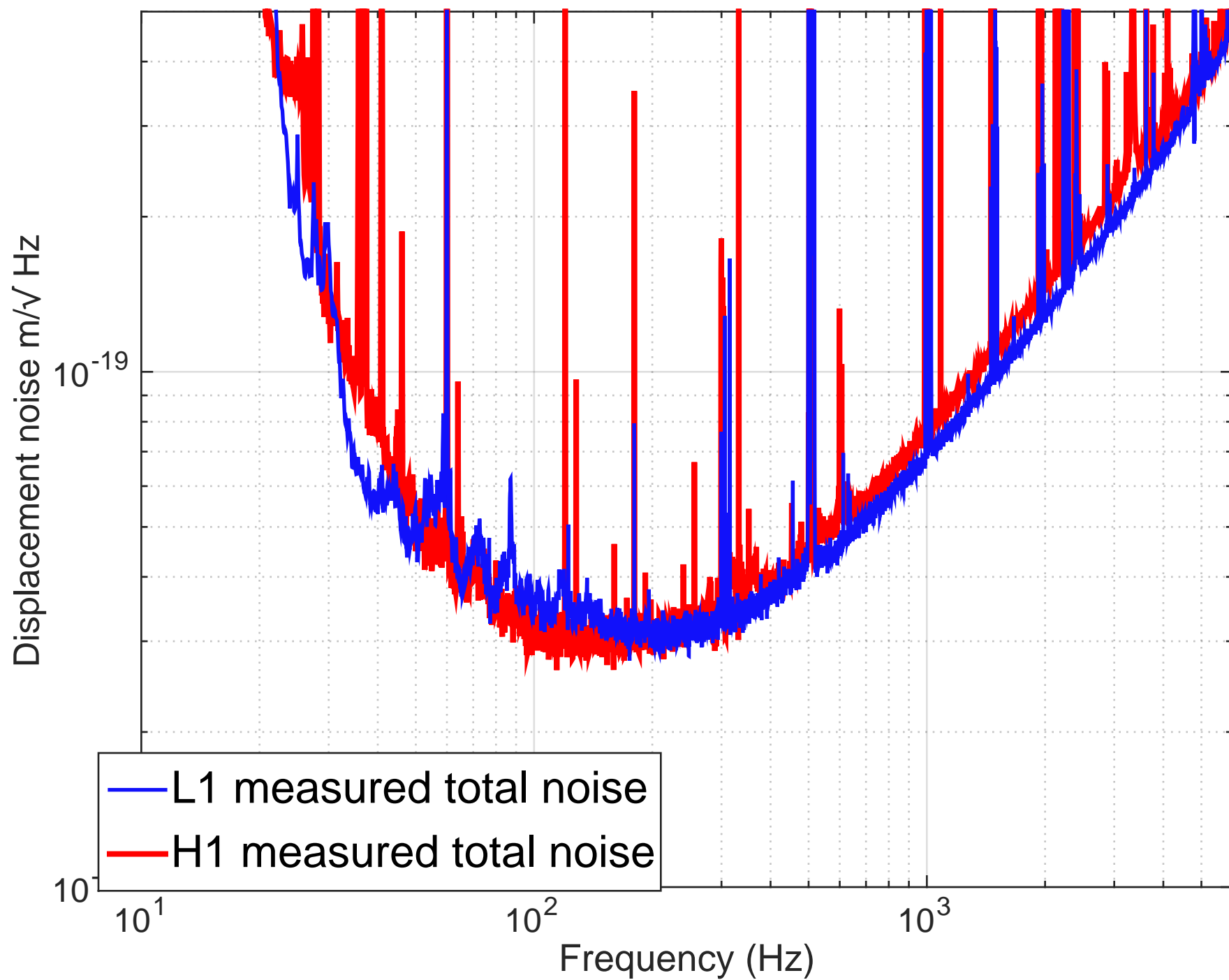
Best L1 and H1 noise curves
