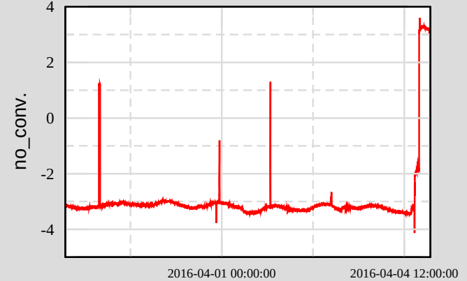
Ch 7: H1:SUS-SR3_M3_OPLEV_YAW_OUTPUT
