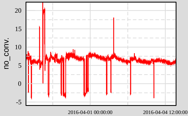
Ch 1: H1:SUS-ETMX_L3_OPLEV_YAW_OUT16
