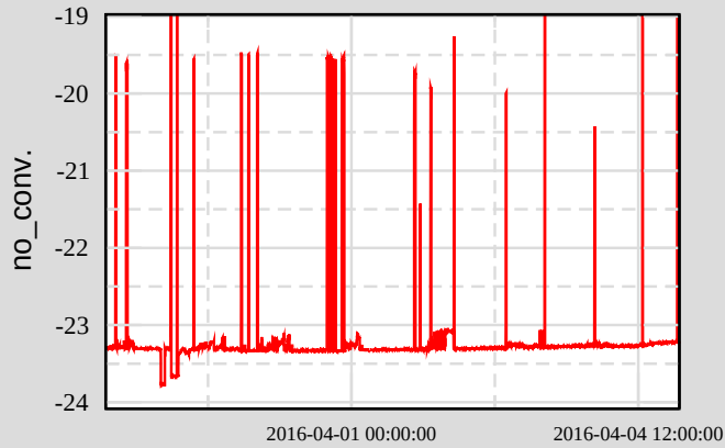
Ch 2: H1:SUS-ETMY_L3_OPLEV_YAW_OUT16
