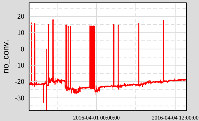
Ch 1: H1:SUS-ETMX_L3_OPLEV_YAW_OUT16
