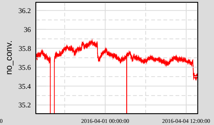
Ch 7: H1:SUS-SR3_M3_OPLEV_YAW_OUTPUT
