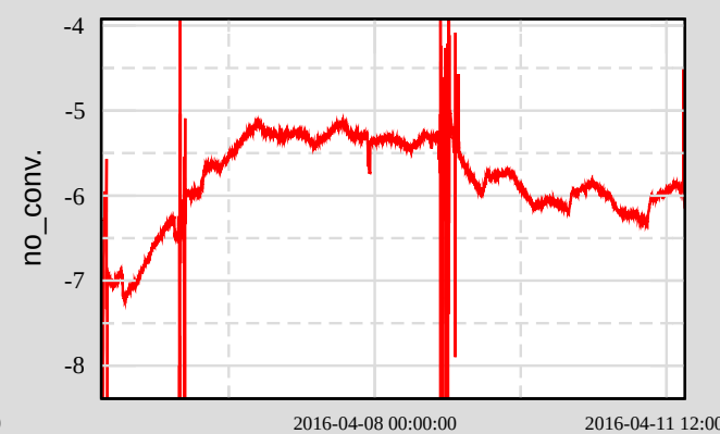
Ch 7: H1:SUS-SR3_M3_OPLEV_PIT_OUT16
