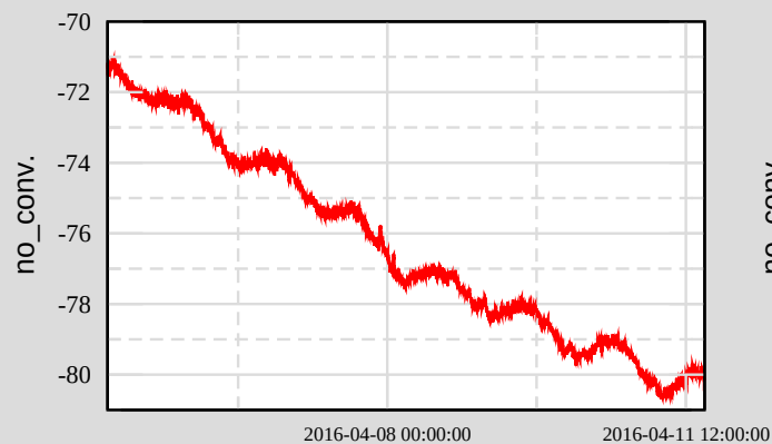
Ch 1: H1:SUS-ETMX_L3_OPLEV_PIT_OUT16
