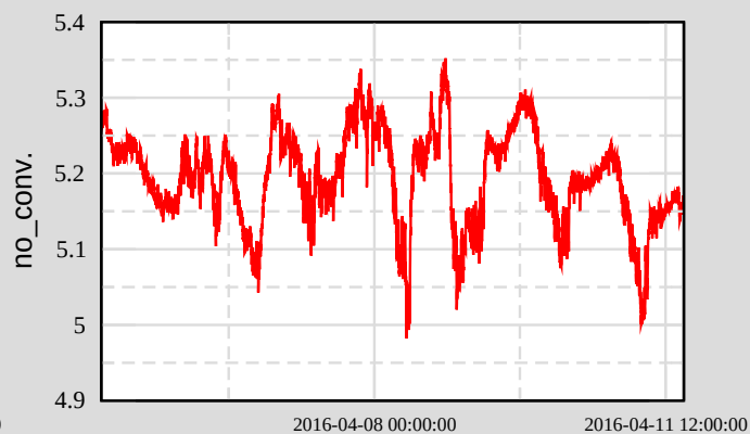
Ch 5: H1:SUS-BS_M3_OPLEV_PIT_OUT16
