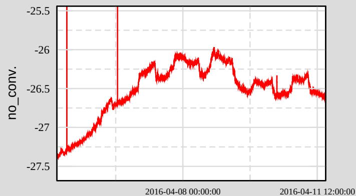
Ch 2: H1:SUS-ETMY_L3_OPLEV_PIT_OUT16
