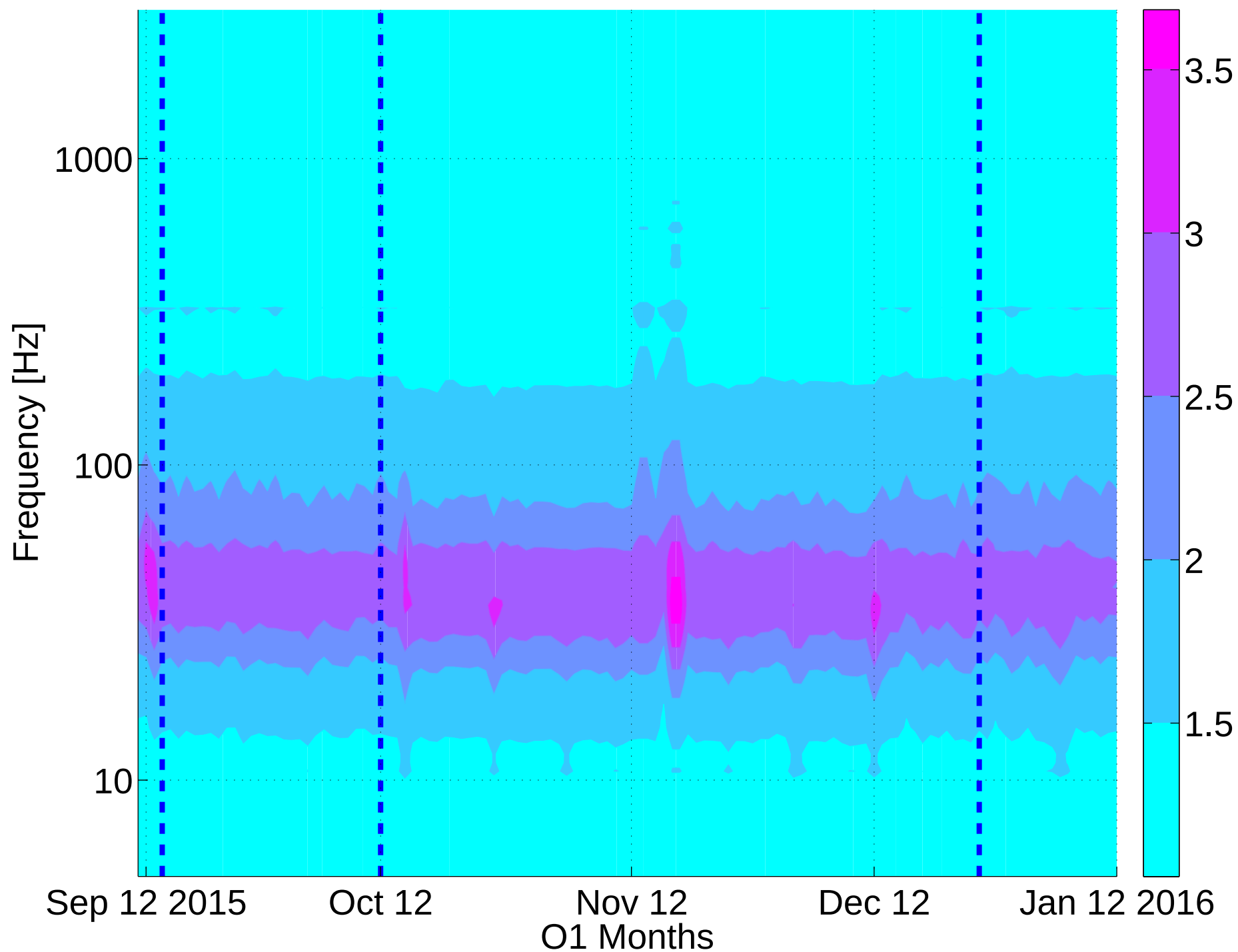
LHO C02 – All of O1 – Phase Statistical Uncertainty
