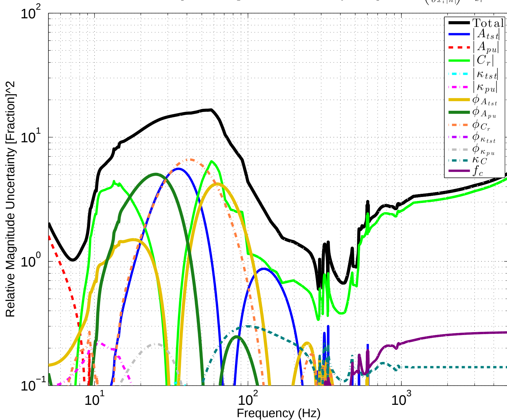
LHO C03 Squared Magnitude Uncertainty Components \left(\frac{\partial |h|}{\partial x_i} \frac{1}{|h|}\right)^2 \sigma_{x_i}^2
