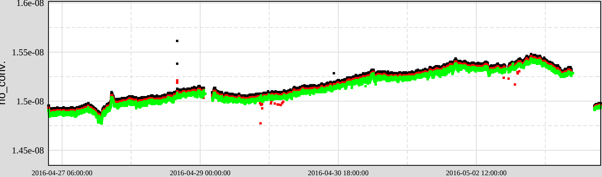
Ch 15: H0:VAC-LX_X2_PT170_MOD1_PRESS_TORR
