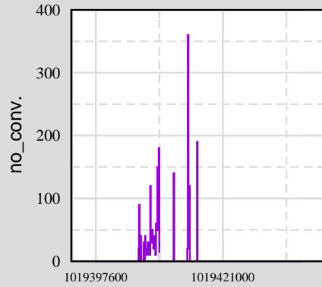
Ch 8: H0:PEM-LVEA_DST14_5
