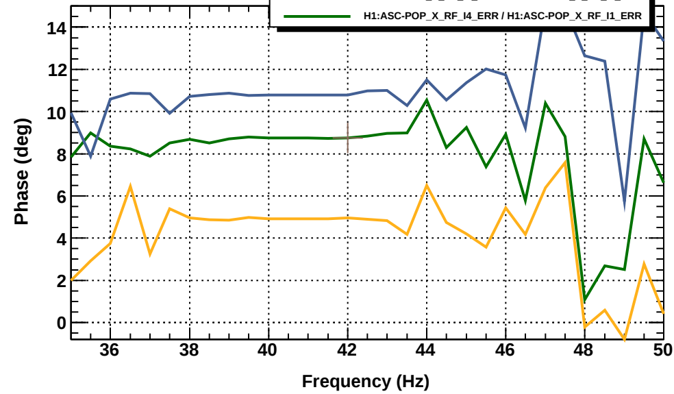
Transfer function
