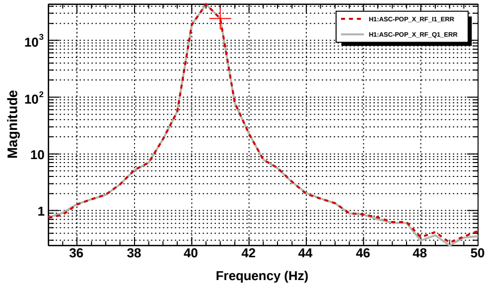
Power spectrum
