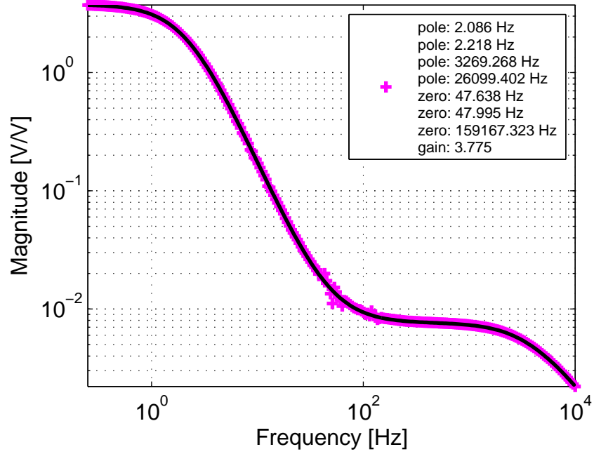
ETMY ESD LVLN driver: UR (measured: 2016-05-06)
