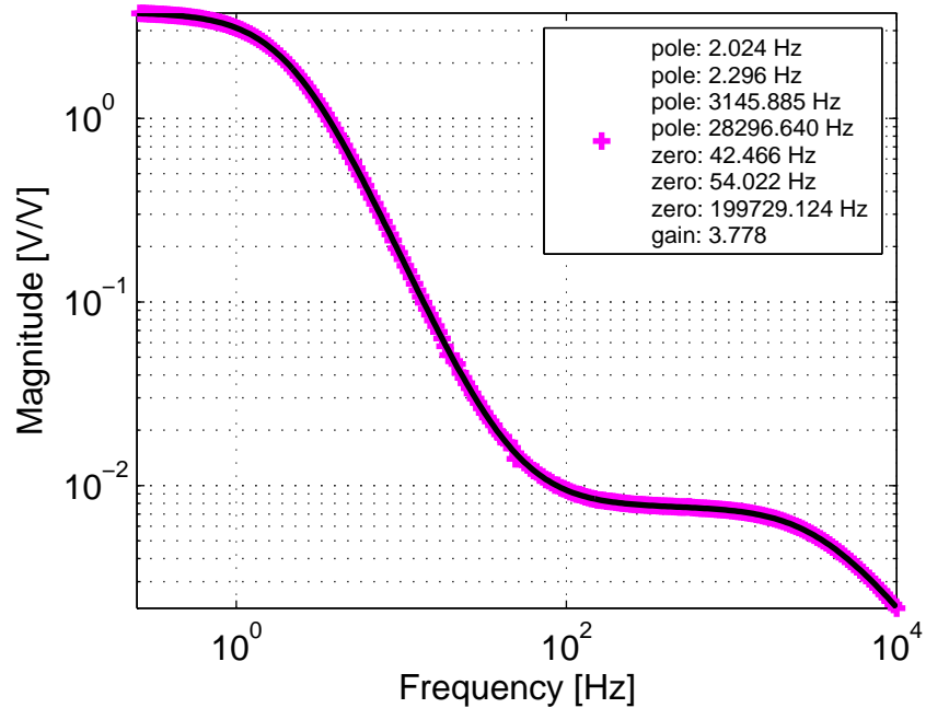
ETMY ESD LVLN driver: UL (measured: 2016-05-06)
