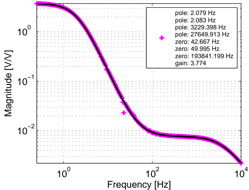
ETMY ESD LVLN driver: LL (measured: 2016-05-06)
