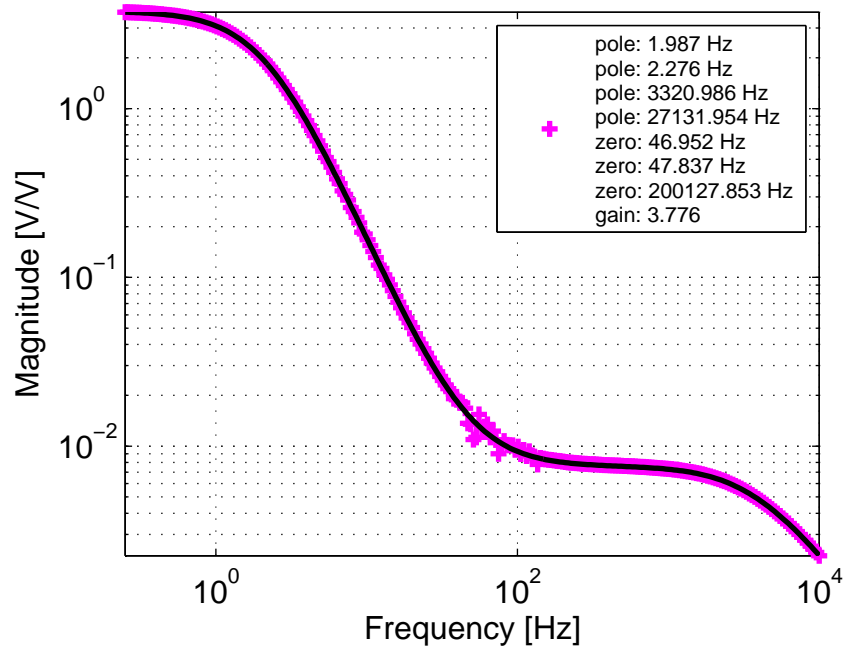
ETMY ESD LVLN driver: LR (measured: 2016-05-06)
