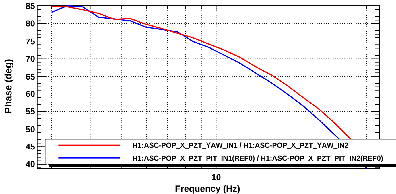
Transfer function
