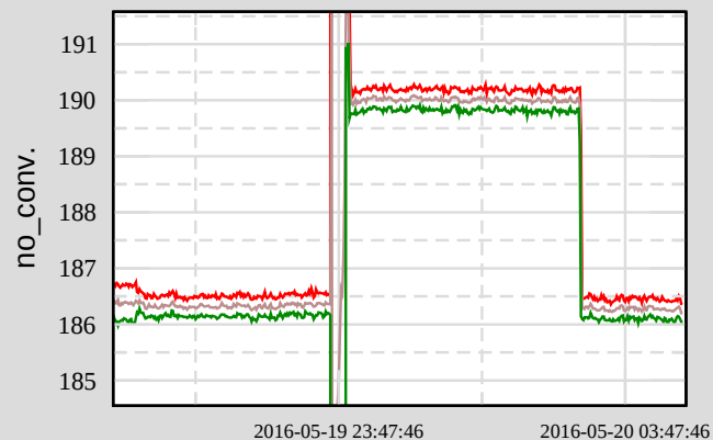
Ch 1: H1:SUS-IM1_M1_DAMP_P_INMON
