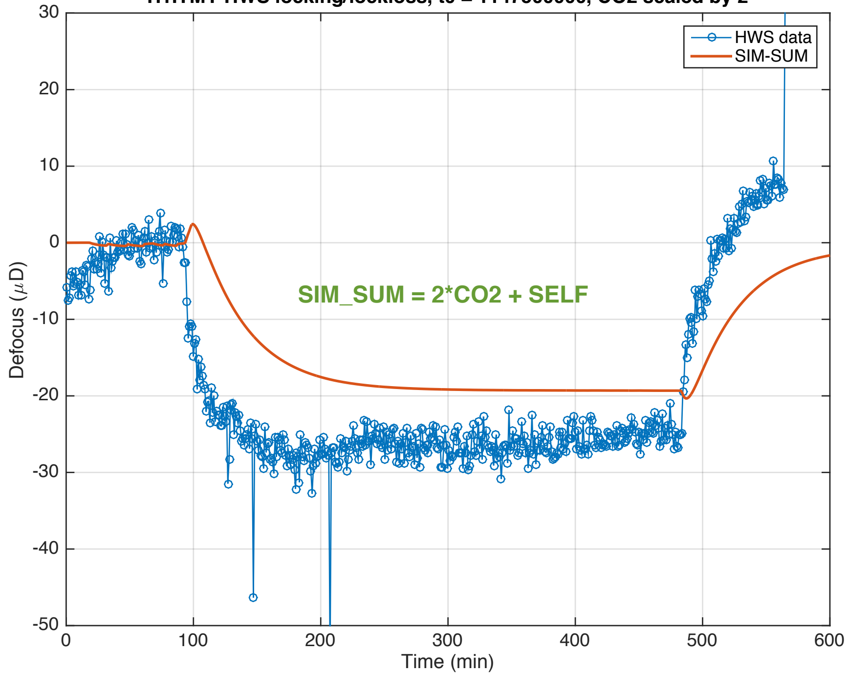
H1ITMY HWS locking/lockloss, t0 = 1147500000, CO2 scaled by 2
