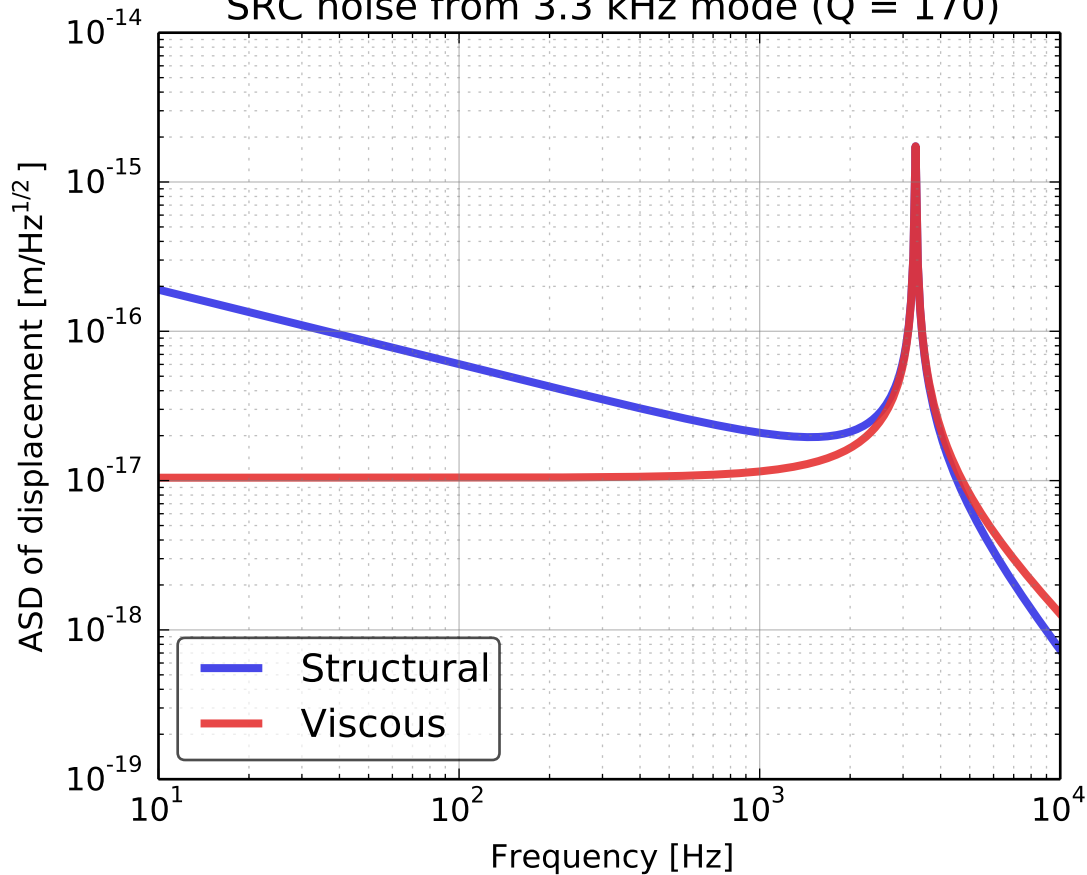
SRC noise from 3.3 kHz mode (Q = 170)
