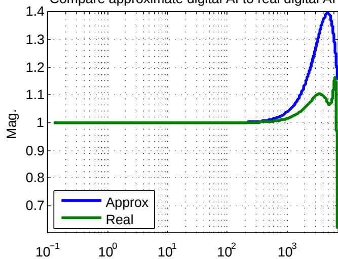
Compare approximate digital AI to real digital AI
