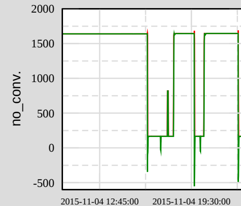
Ch 10: H1:ISI-HAM5_OPLEV_SUM_OUT16
