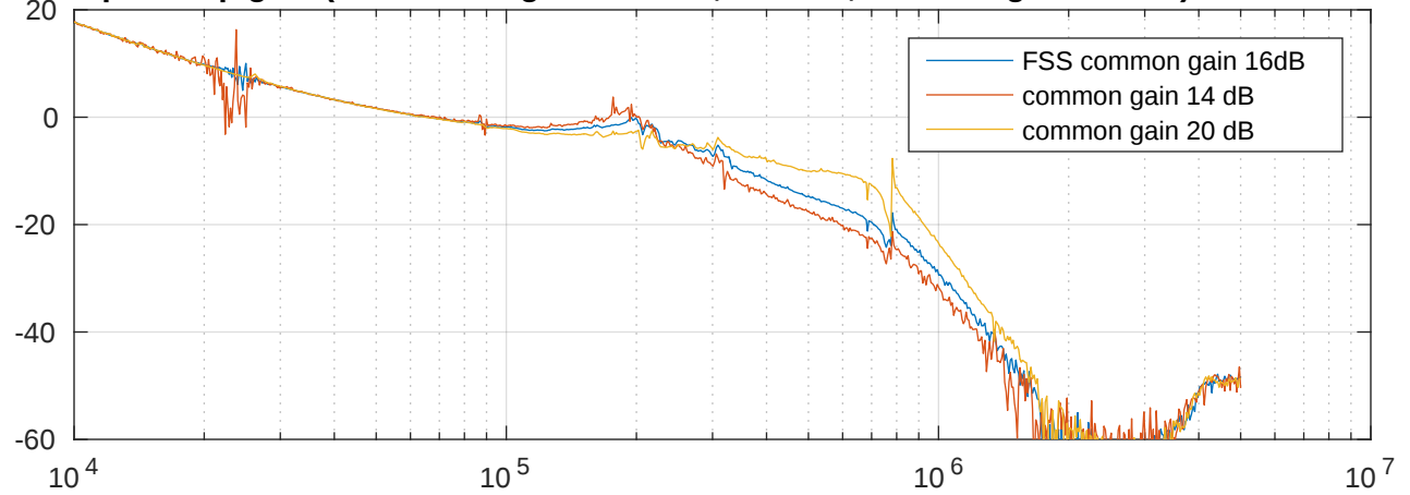
IMC open loop gain (IMC refl in1 gain = 16 dB, 2 Watts, FSS fast gain 22.2dB)
