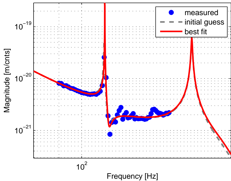
UIM transfer function
