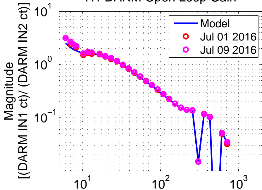
H1 DARM Open Loop Gain
