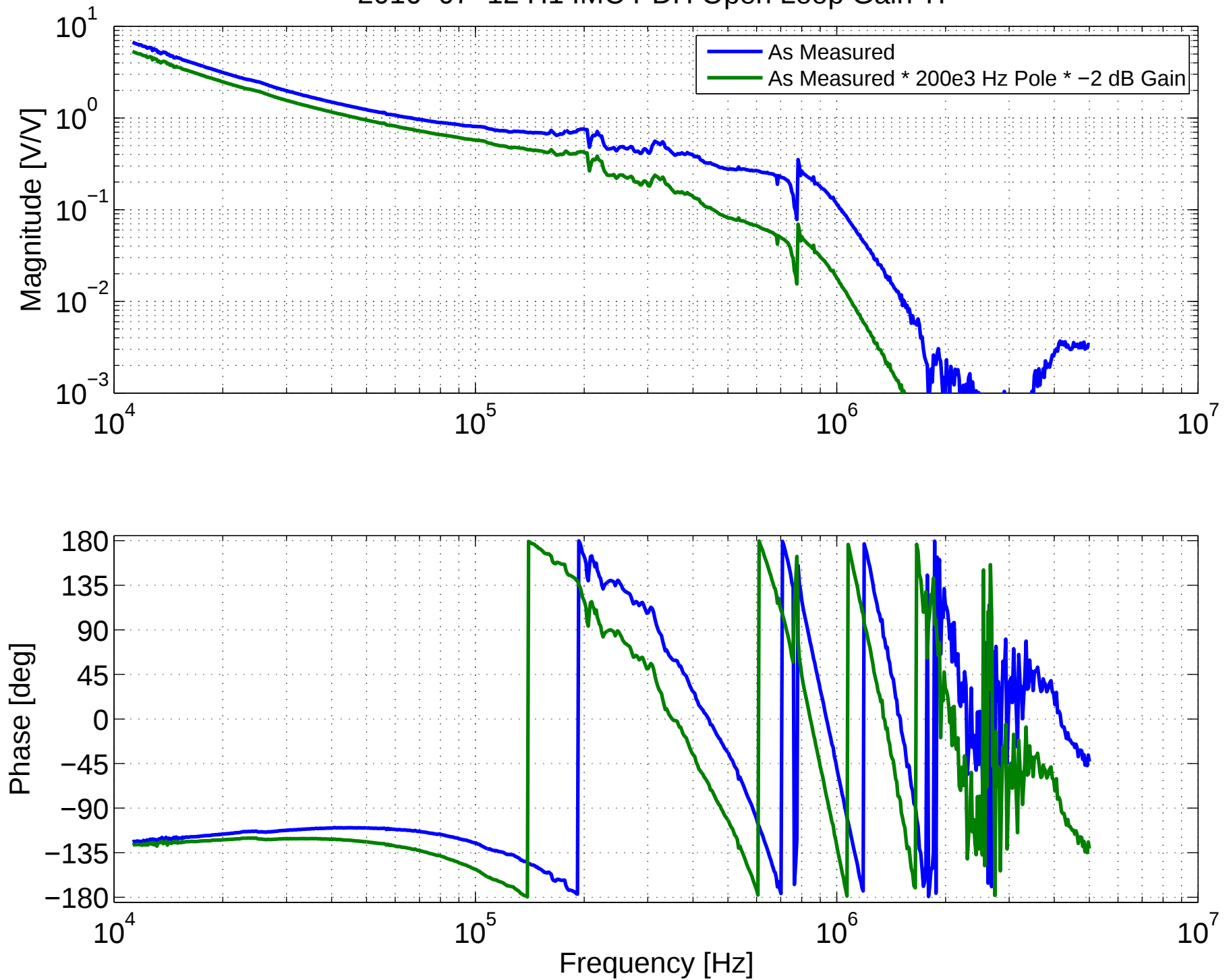
2016-07-12 H1 IMC PDH Open Loop Gain TF
