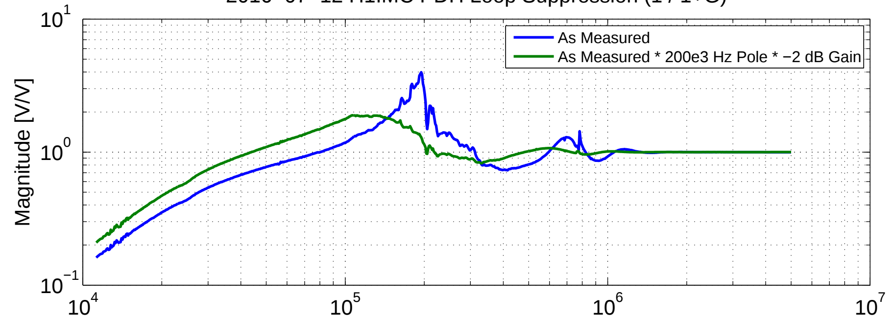
2016-07-12 H1IMC PDH Loop Suppression ( 1 / 1+G )
