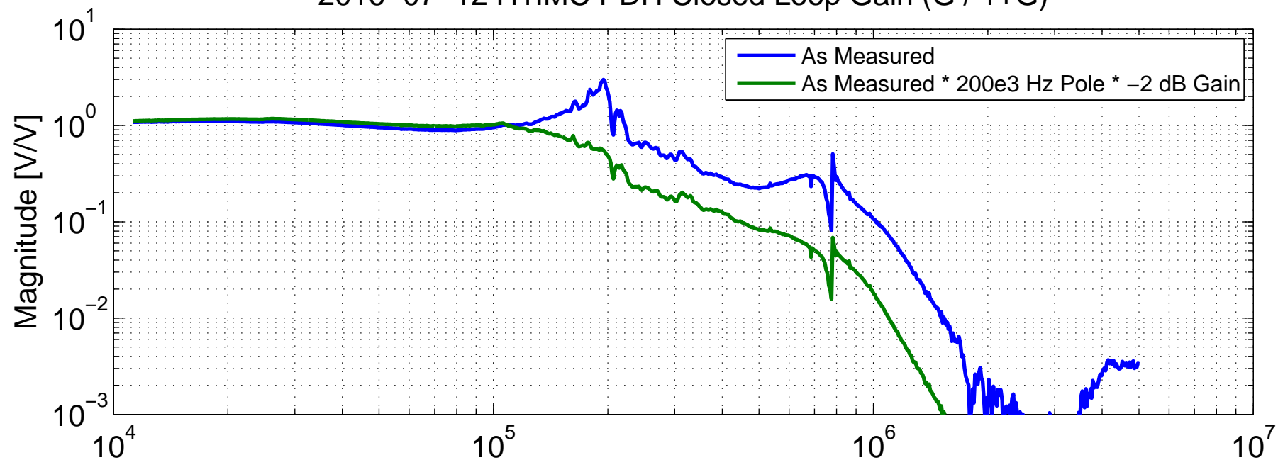
2016-07-12 H1IMC PDH Closed Loop Gain ( G / 1+G )
