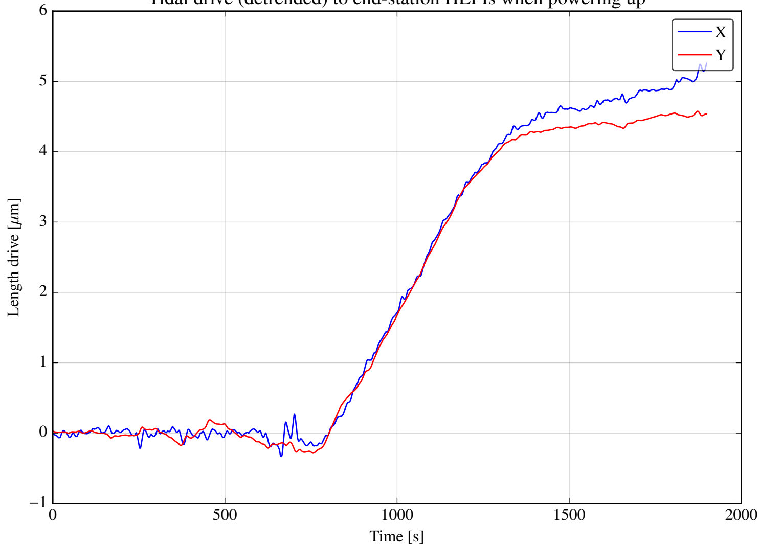
Tidal drive (detrended) to end-station HEPIs when powering up
