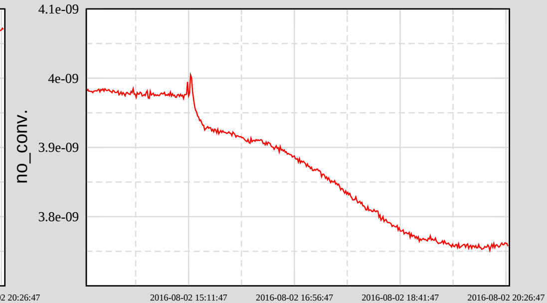
Ch 4: H0:VAC-LX_X3_PT134B_PRESS_TORR
