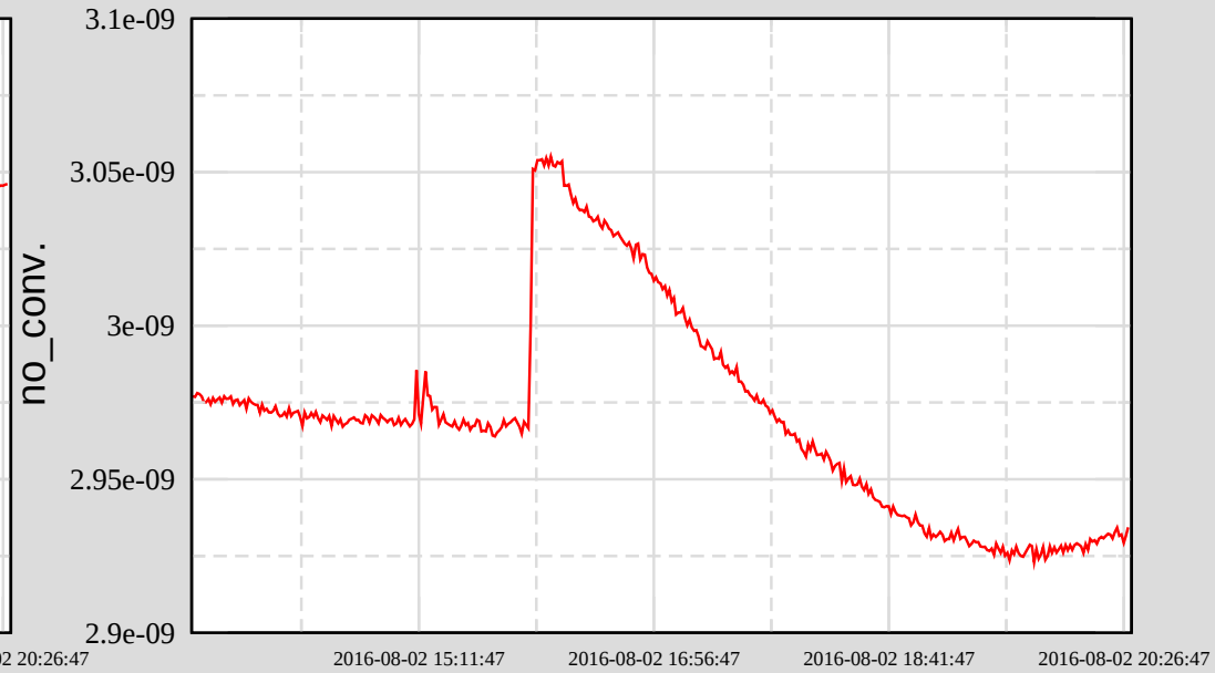
Ch 5: H0:VAC-LX_X4_PT144B_PRESS_TORR
