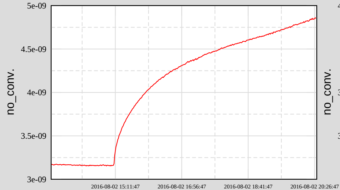
Ch 2: H0:VAC-LY_Y4_PT124B_PRESS_TORR
