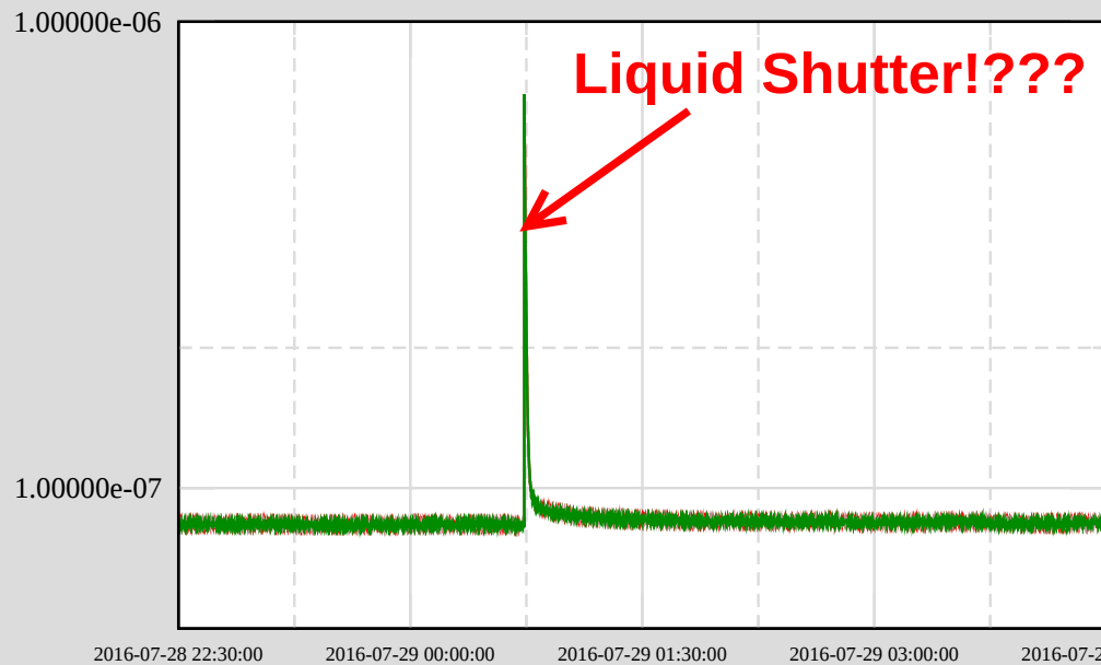
Ch 2: H0:VAC-LX_Y0_PT110B_PRESS_TORR
