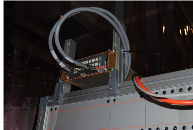
Shutter Logic Box Used to reside on Table. Moved to Rack to reduce need to make and remove connections.
