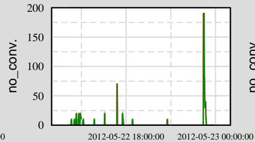
Ch 9: H0:PEM-EY_DST1_5
