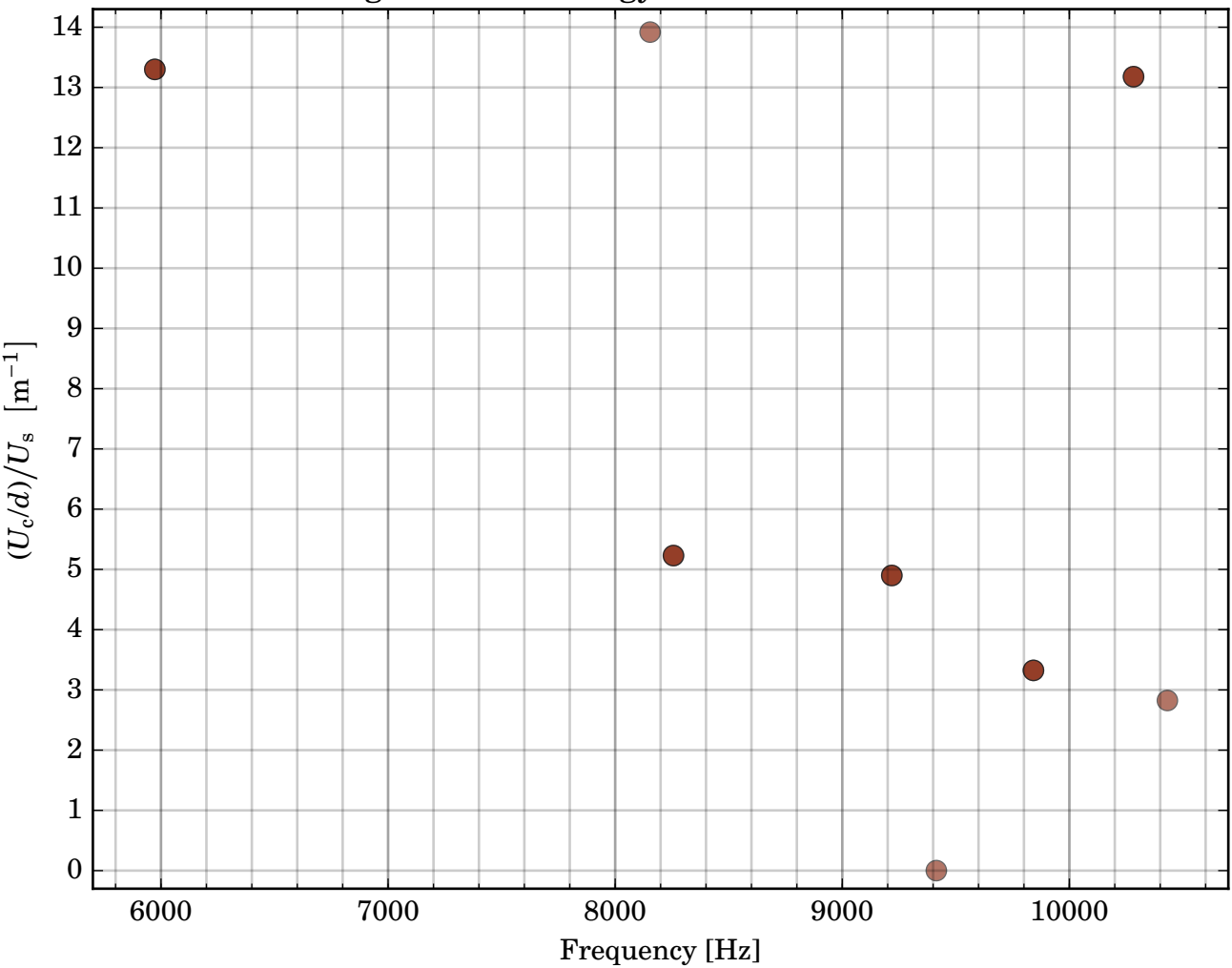
Coating/substrate energy ratio for test mass modes
