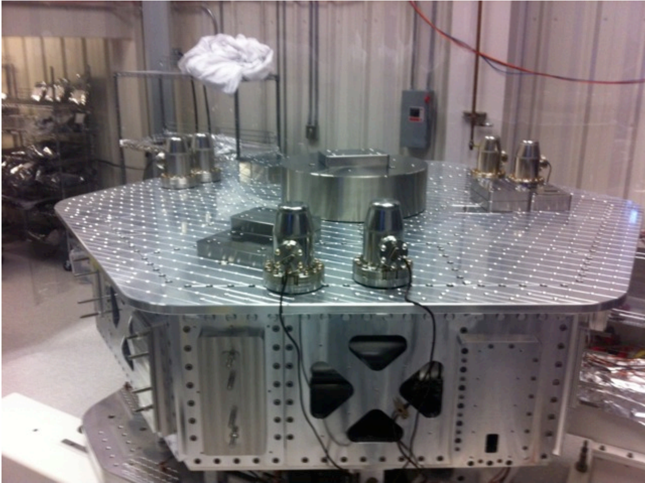
Testing set up – L4Cs wired up to GS13s pigtail cables
