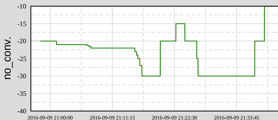
Ch 8: H1:PSL-ISS_DIFFRACTION_AVG
