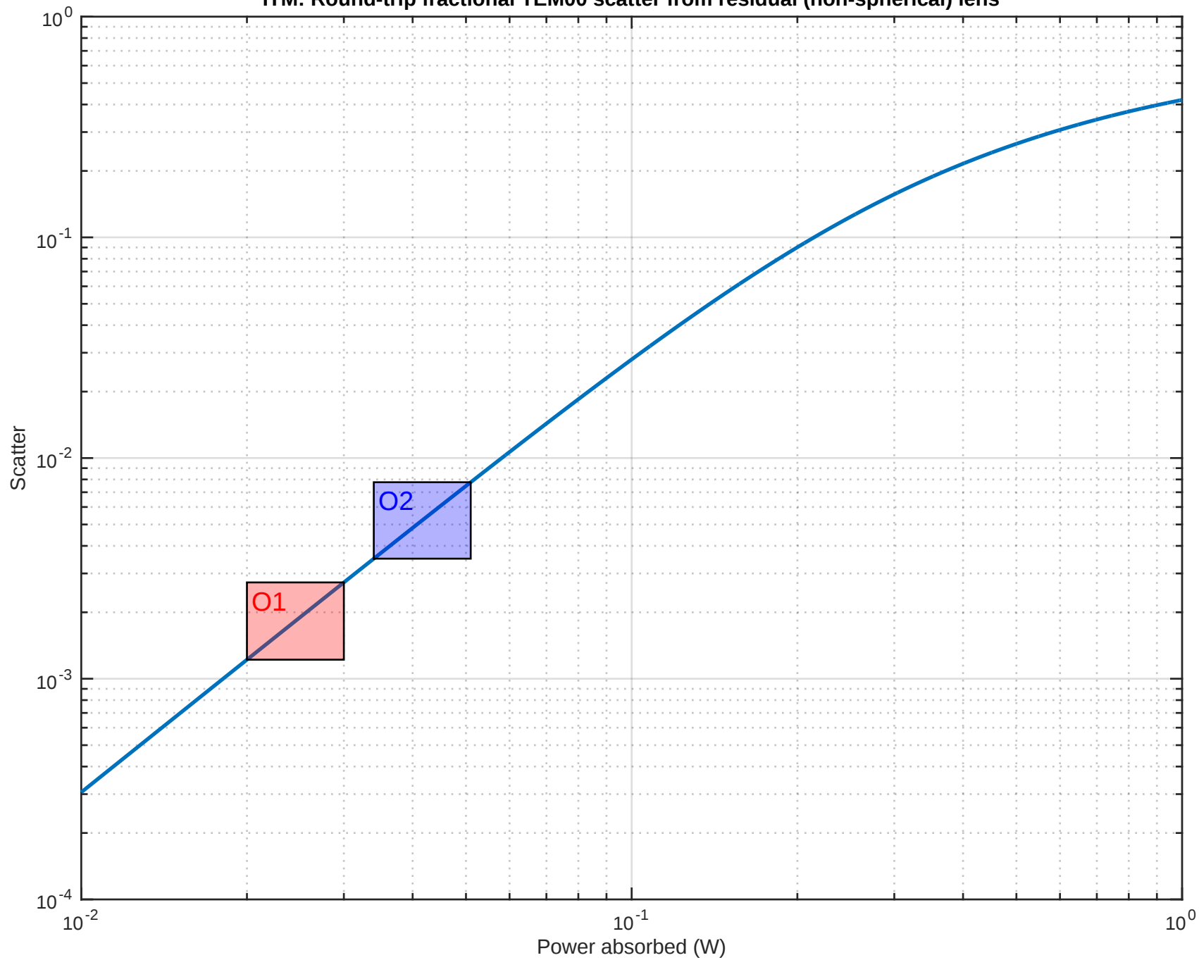
ITM: Round-trip fractional TEM00 scatter from residual (non-spherical) lens
