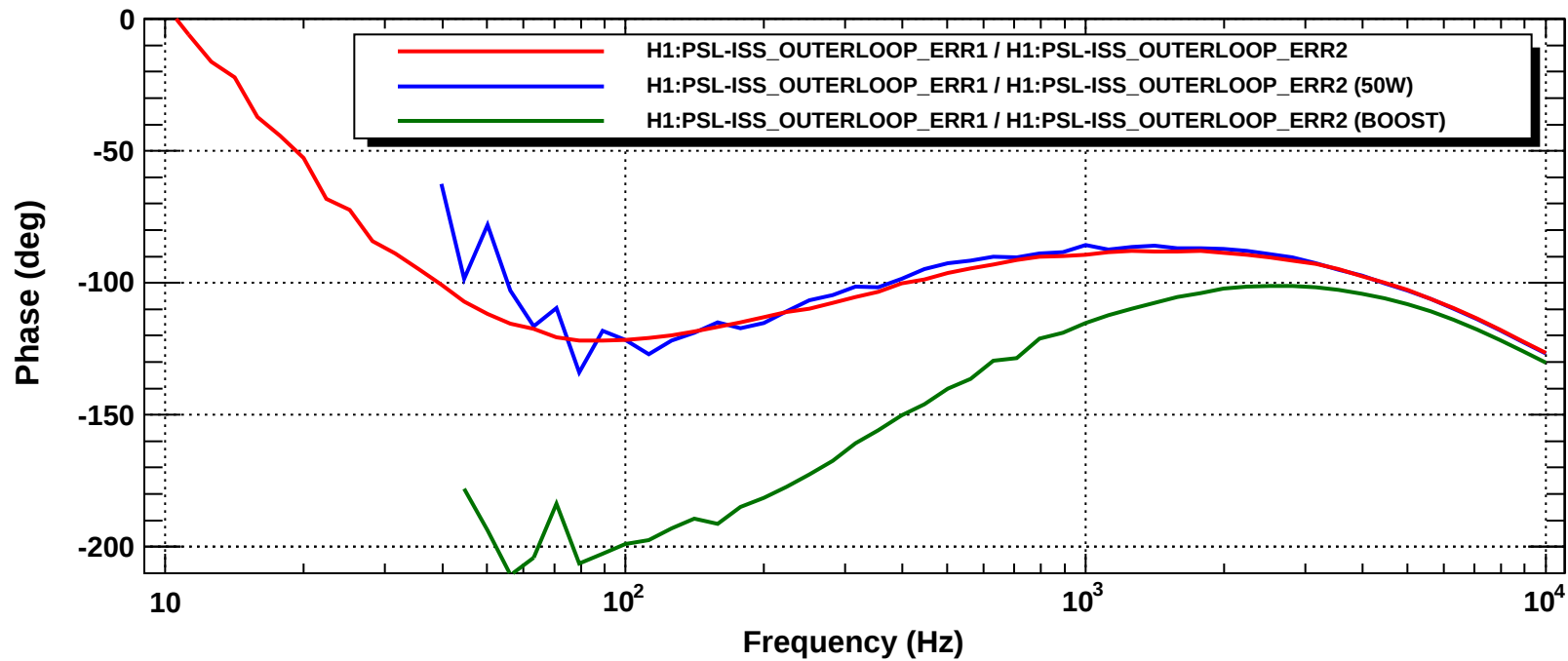
Transfer function
