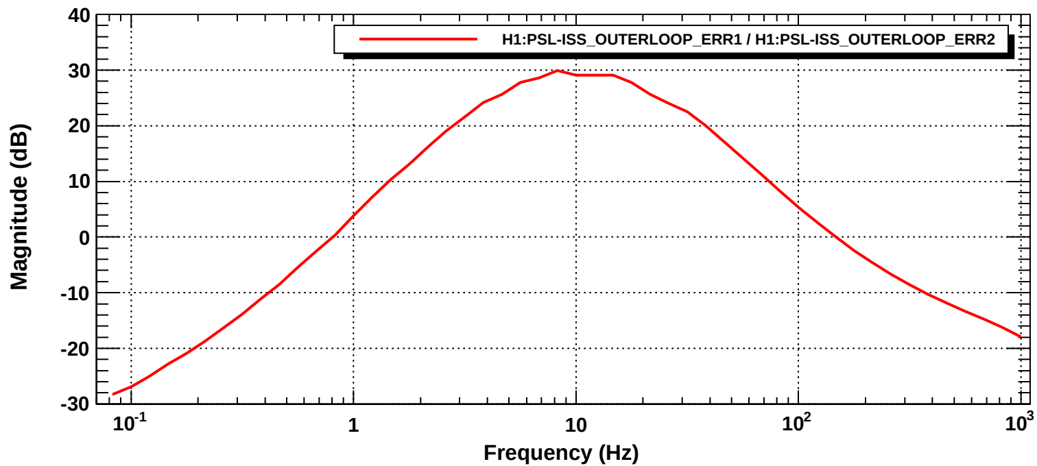
Transfer function
