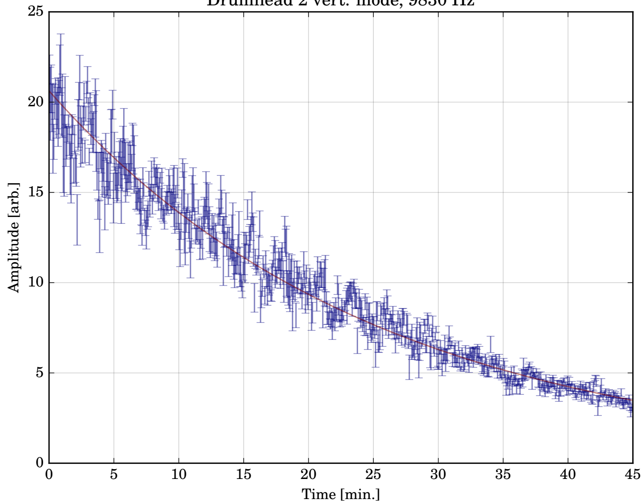
Drumhead 2 vert. mode, 9830 Hz
