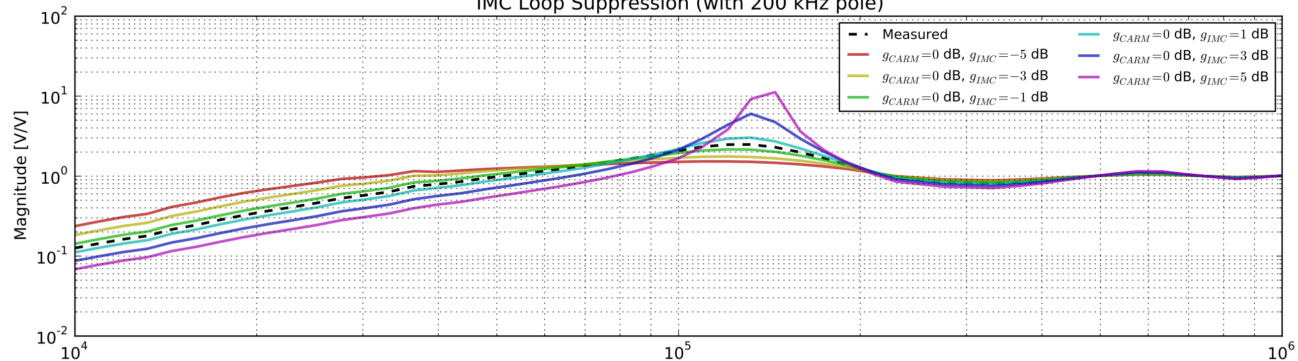
IMC Loop Suppression (with 200 kHz pole)
