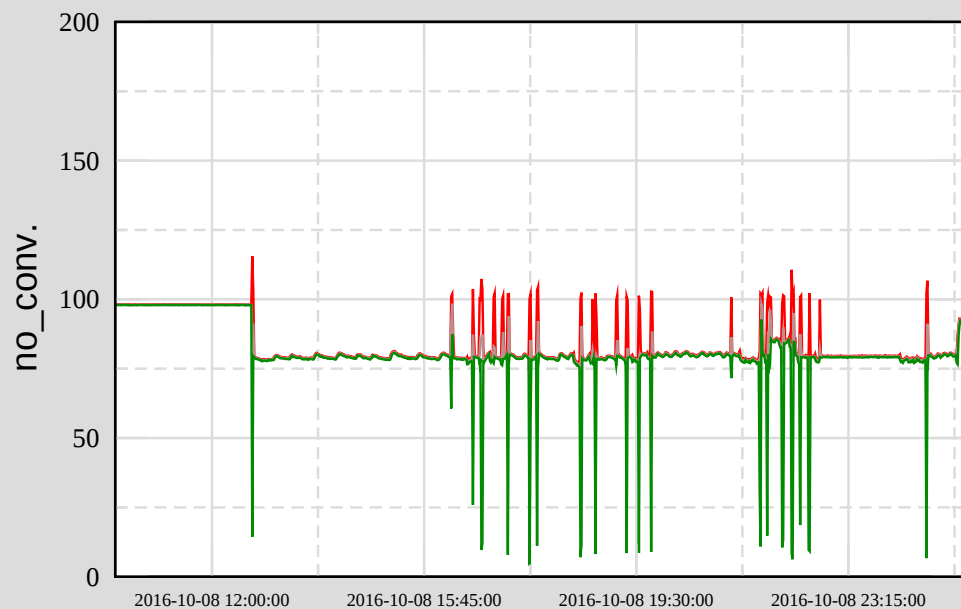
Ch 1: H1:PSL-PWR_PMC_TRANS_OUTPUT
