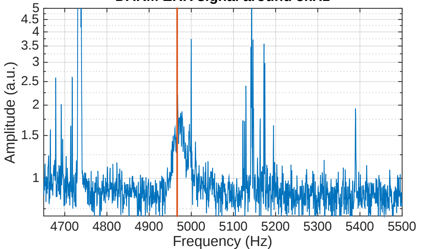
DARM ERR signal around 5kHz
