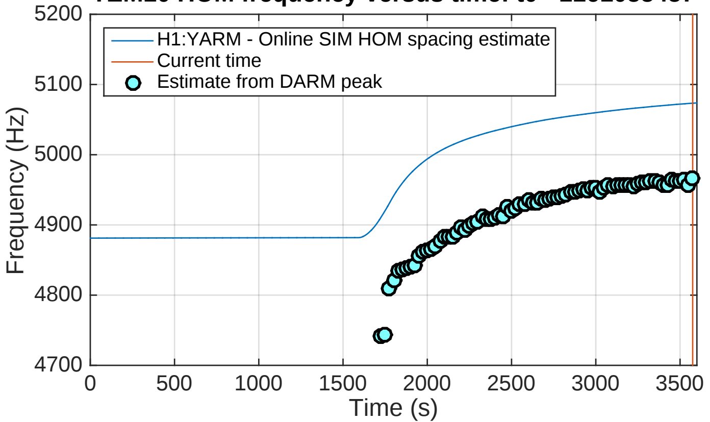
TEM10 HOM frequency versus time: t0 =1161055457
