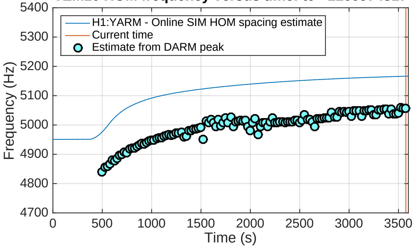
TEM10 HOM frequency versus time: t0 =1160974817
