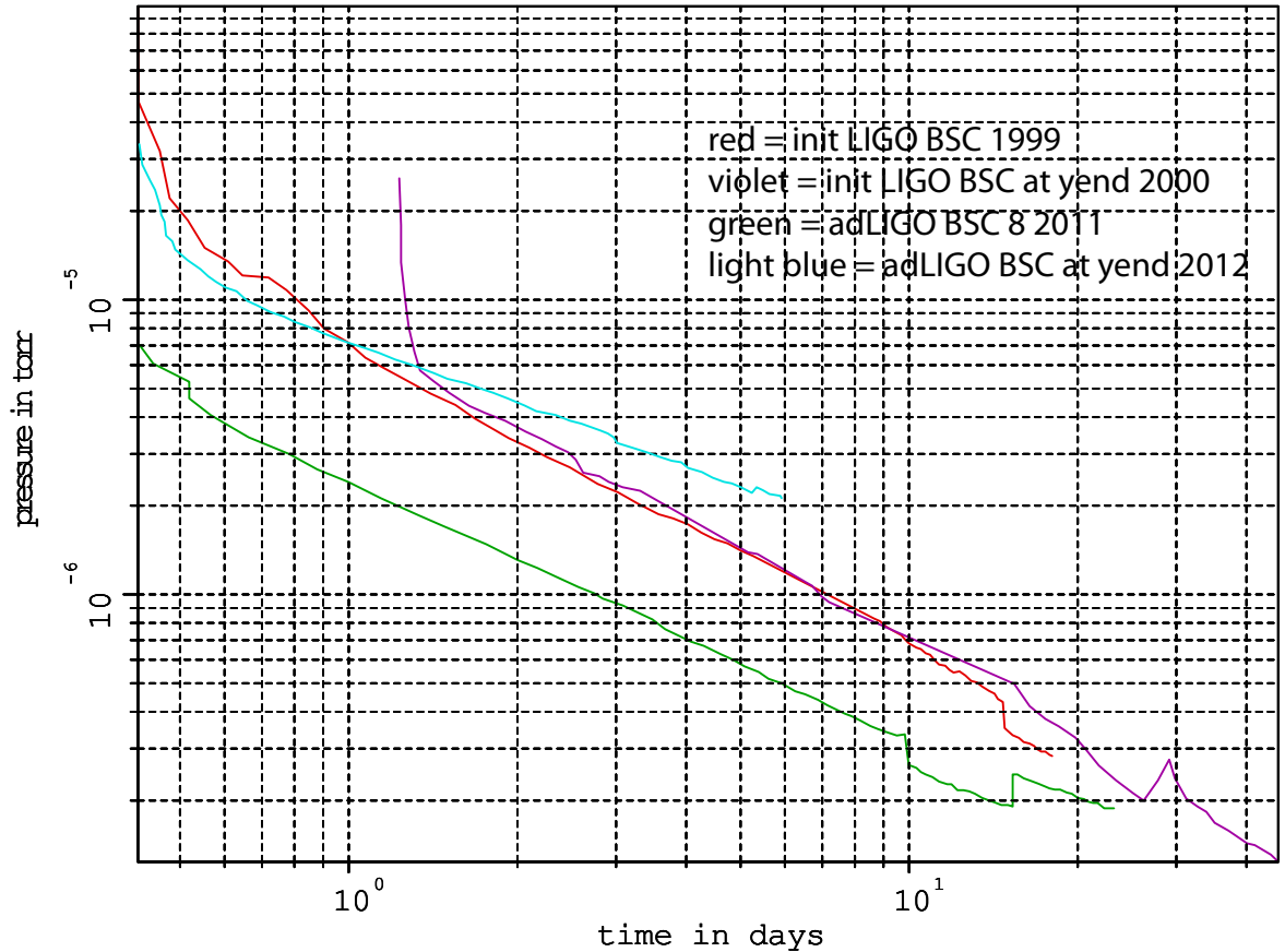
initial and advanced LIGO BSC pumpdown curves
